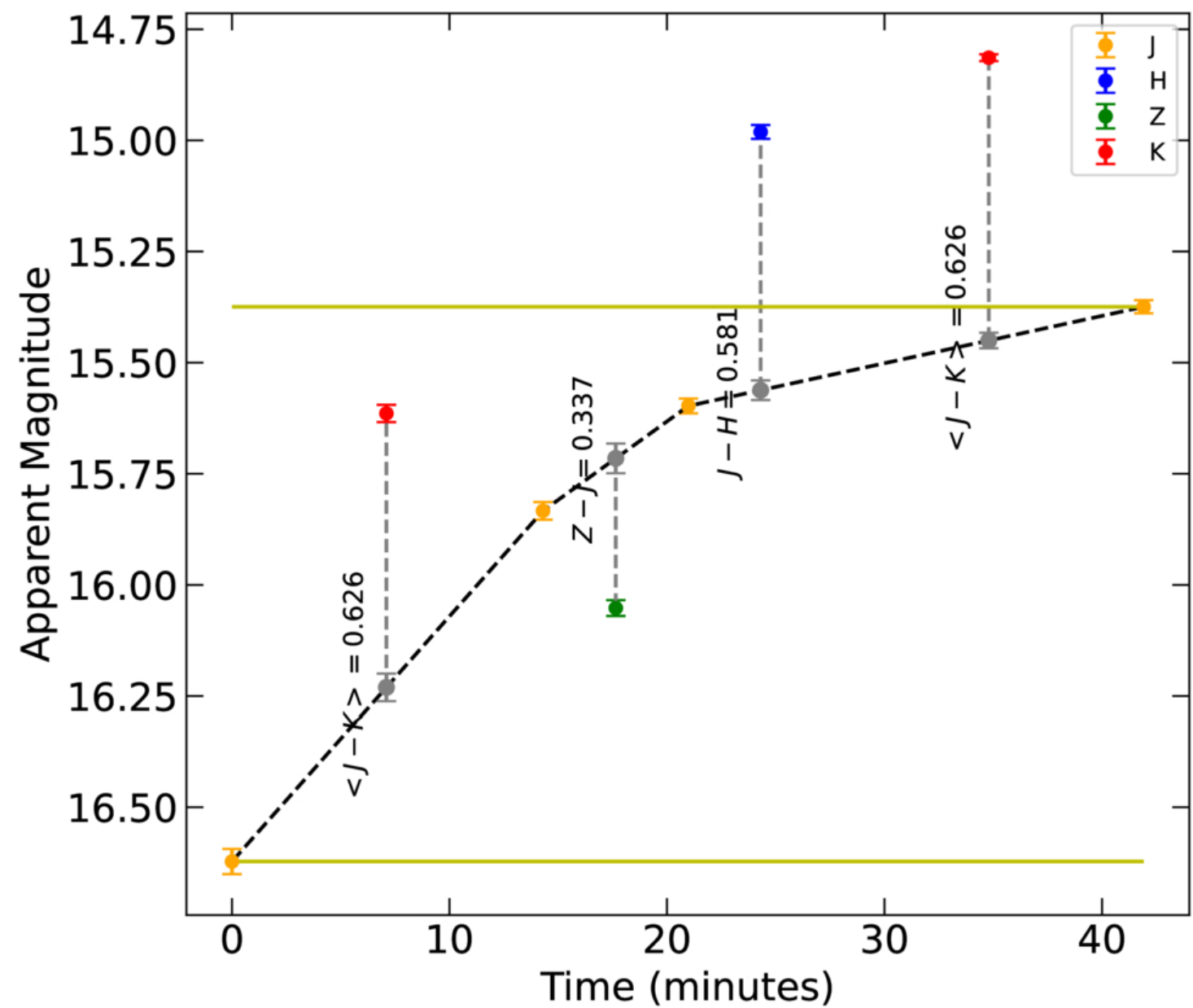
Figure 1. from Andy J. López-Oquendo et al 2026 Planet. Sci. J. 7 doi:10.3847/PSJ/ae9f3f https://dx.doi.org/10.3847/PSJ/ae9f3f © 2026. The Author(s). Published by the American Astronomical Society.
