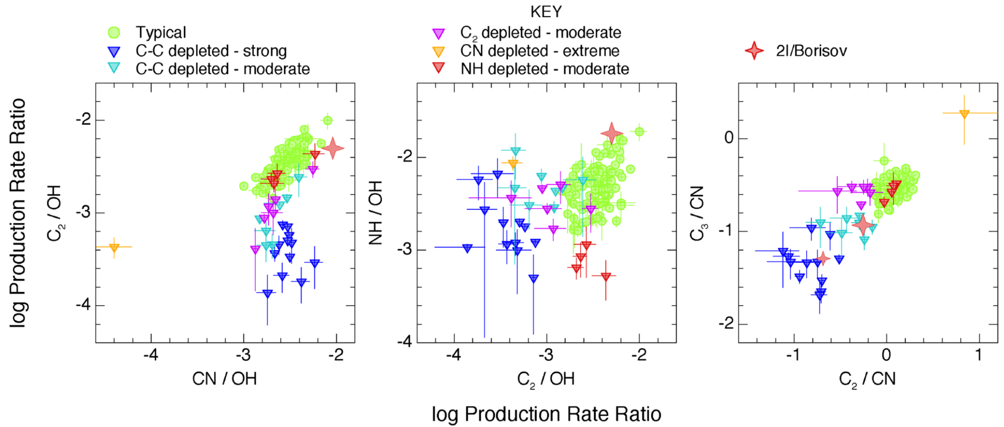
Figure 7. from Allison N. Bair et al 2026 Planet. Sci. J. 7 doi:10.3847/PSJ/ae9f3d https://dx.doi.org/10.3847/PSJ/ae9f3d © 2026. The Author(s). Published by the American Astronomical Society.
