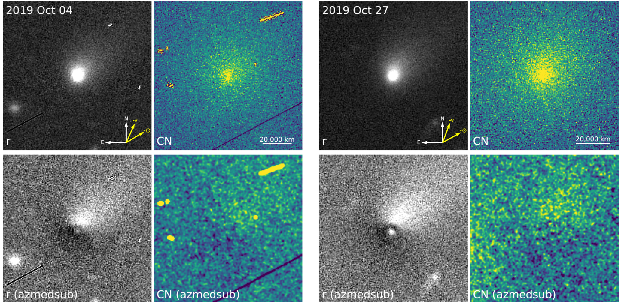
Figure 3. from Allison N. Bair et al 2026 Planet. Sci. J. 7 doi:10.3847/PSJ/ae9f3d https://dx.doi.org/10.3847/PSJ/ae9f3d © 2026. The Author(s). Published by the American Astronomical Society.
