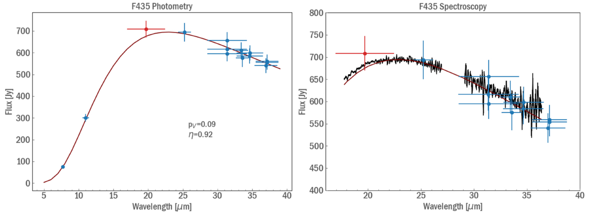
Figure A1. NEATM photometric and spectral fits from Anicia Arredondo et al 2026 Planet. Sci. J. 7 doi:10.3847/PSJ/ae9ec4 https://dx.doi.org/10.3847/PSJ/ae9ec4 © 2026. The Author(s). Published by the American Astronomical Society.
