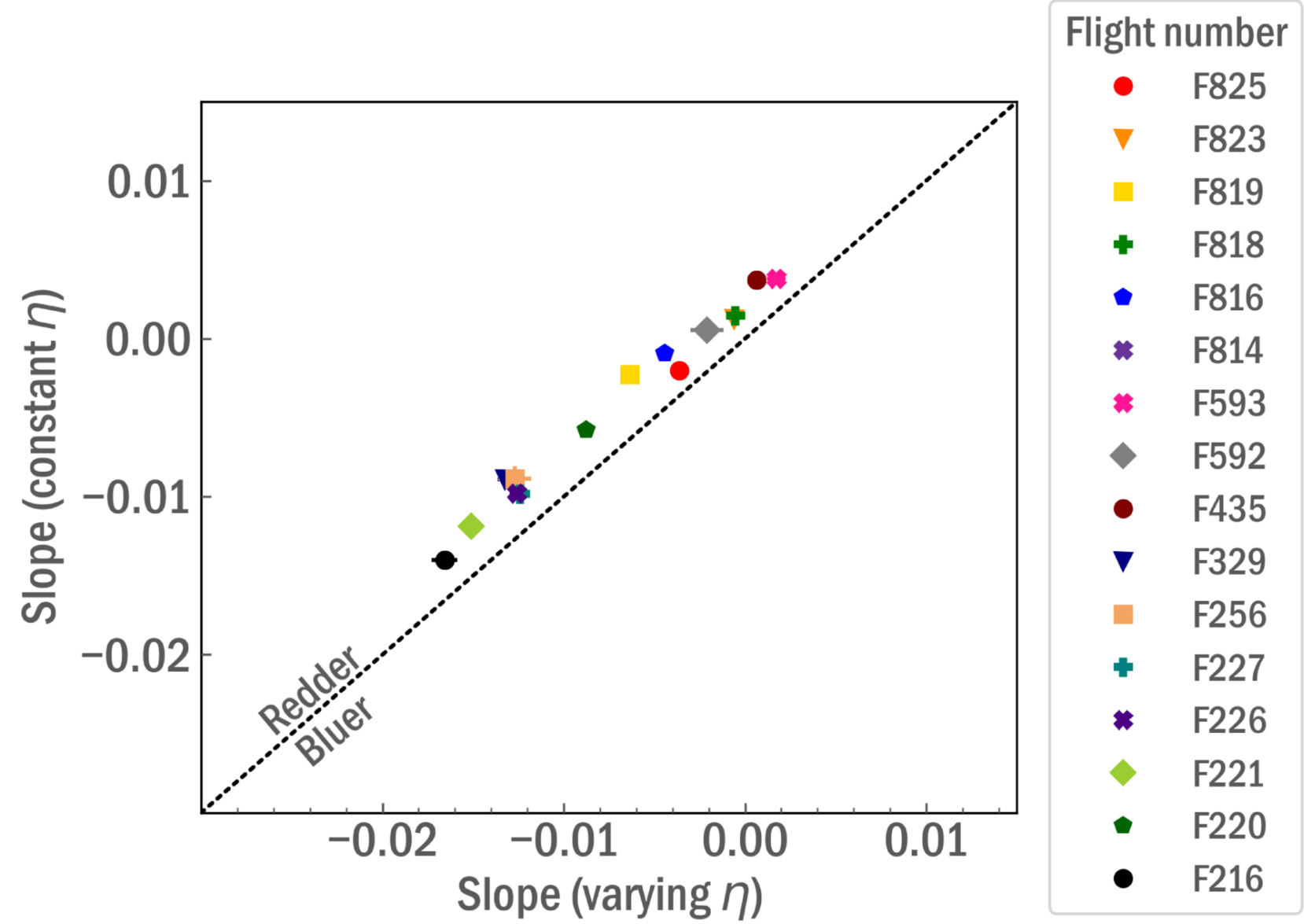
Figure 8. from Anicia Arredondo et al 2026 Planet. Sci. J. 7 doi:10.3847/PSJ/ae9ec4 https://dx.doi.org/10.3847/PSJ/ae9ec4 © 2026. The Author(s). Published by the American Astronomical Society.
