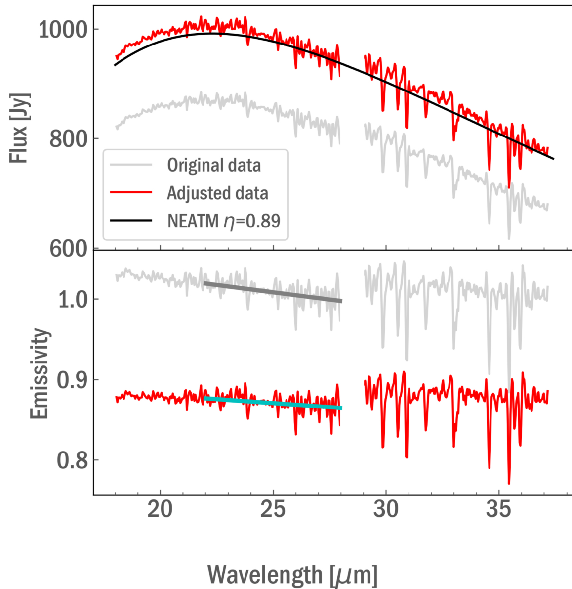
Figure 7. from Anicia Arredondo et al 2026 Planet. Sci. J. 7 doi:10.3847/PSJ/ae9ec4 https://dx.doi.org/10.3847/PSJ/ae9ec4 © 2026. The Author(s). Published by the American Astronomical Society.
