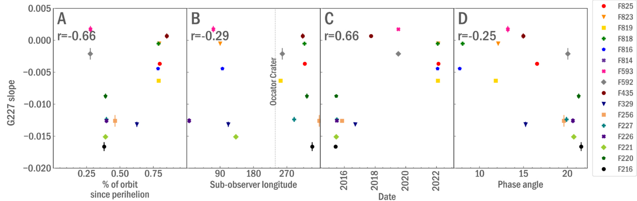
Figure 6. from Anicia Arredondo et al 2026 Planet. Sci. J. 7 doi:10.3847/PSJ/ae9ec4 https://dx.doi.org/10.3847/PSJ/ae9ec4 © 2026. The Author(s). Published by the American Astronomical Society.
