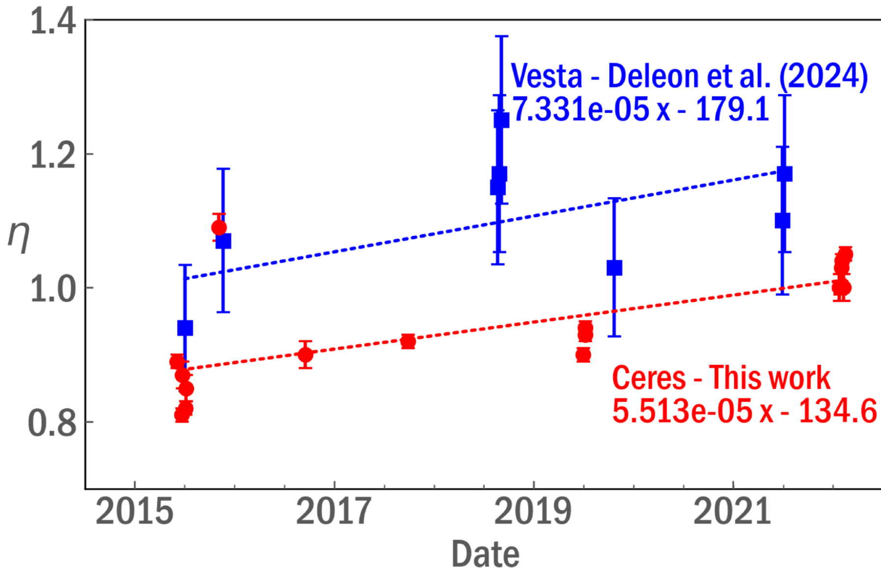
Figure 5. from Anicia Arredondo et al 2026 Planet. Sci. J. 7 doi:10.3847/PSJ/ae9ec4 https://dx.doi.org/10.3847/PSJ/ae9ec4 © 2026. The Author(s). Published by the American Astronomical Society.
