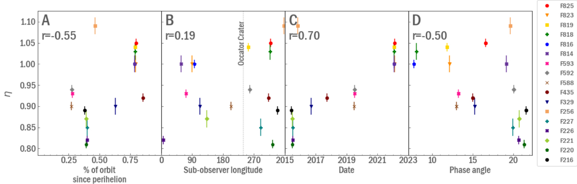
Figure 4. from Anicia Arredondo et al 2026 Planet. Sci. J. 7 doi:10.3847/PSJ/ae9ec4 https://dx.doi.org/10.3847/PSJ/ae9ec4 © 2026. The Author(s). Published by the American Astronomical Society.
