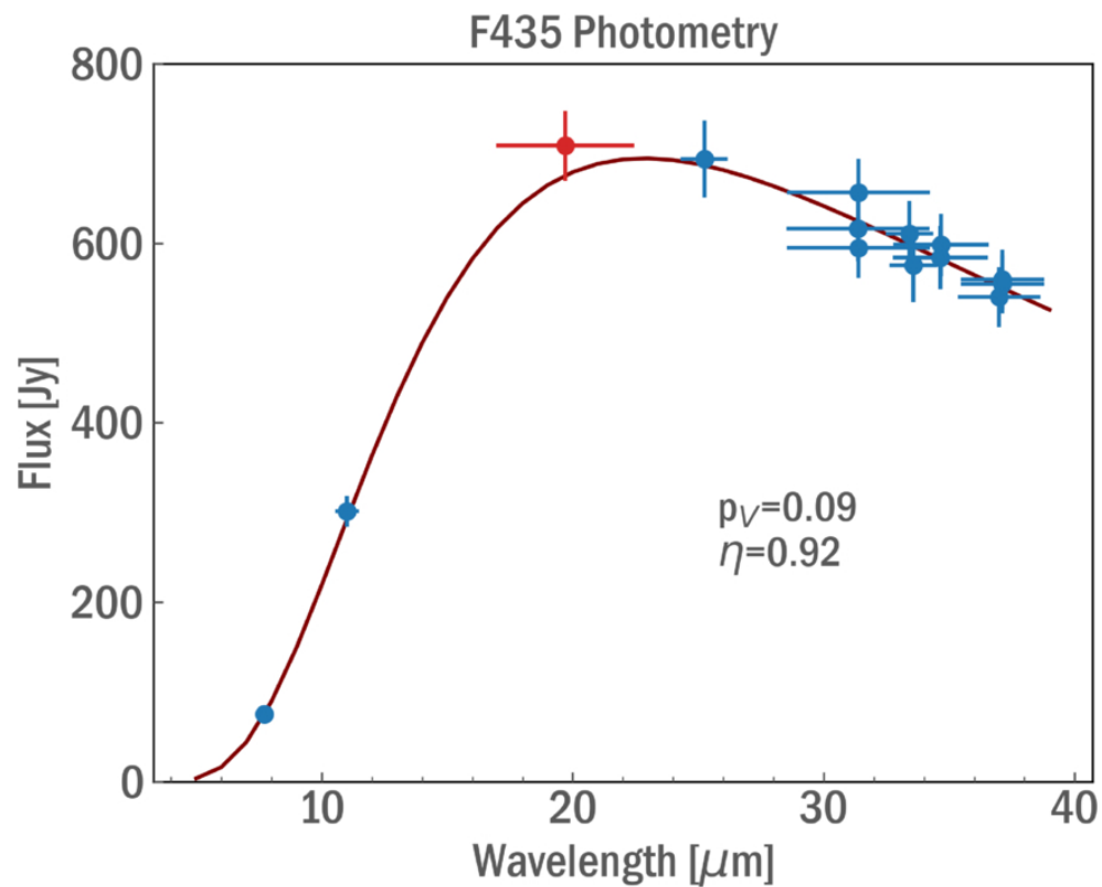
Figure 2. from Anicia Arredondo et al 2026 Planet. Sci. J. 7 doi:10.3847/PSJ/ae9ec4 https://dx.doi.org/10.3847/PSJ/ae9ec4 © 2026. The Author(s). Published by the American Astronomical Society.
