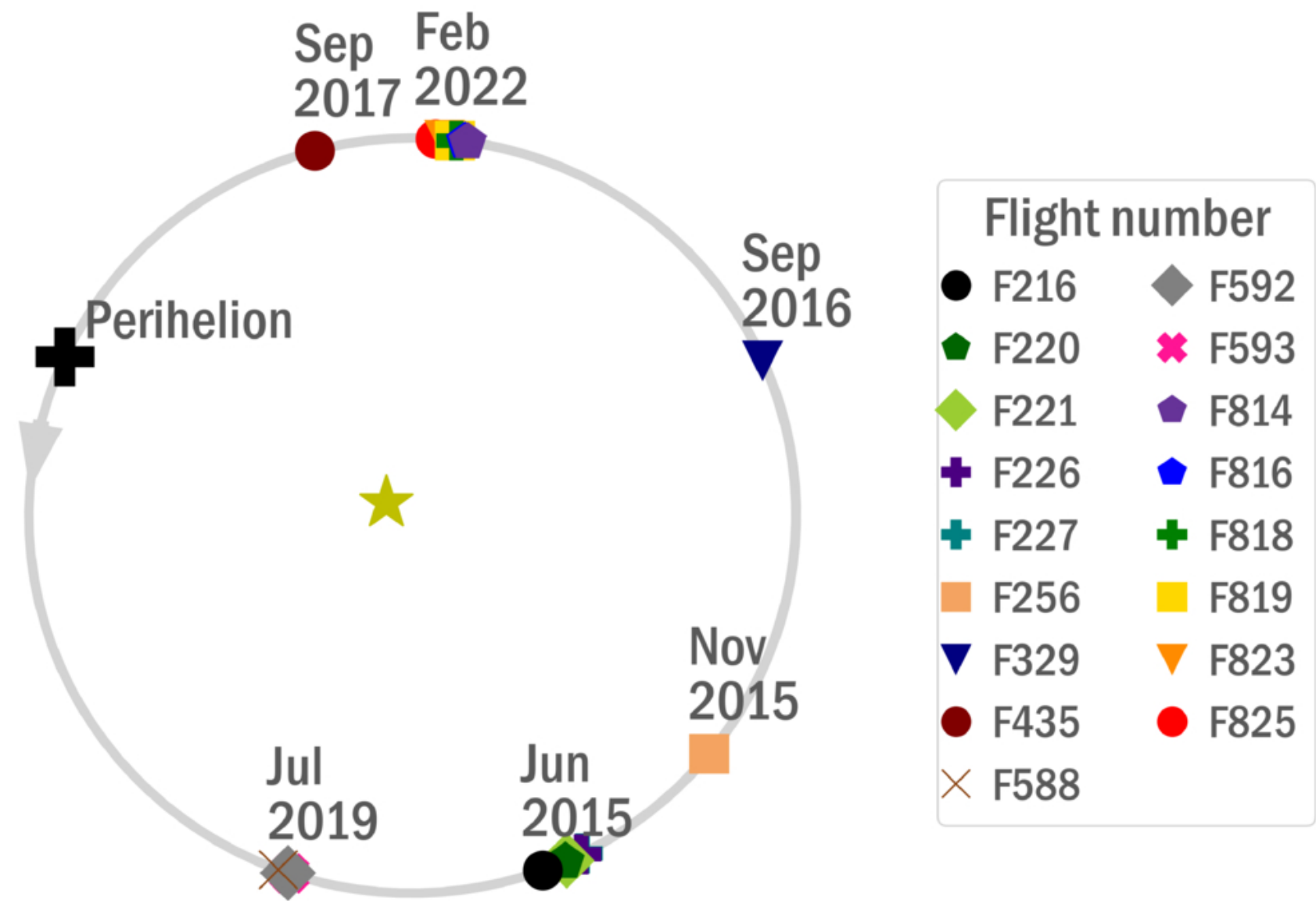
Figure 1. from Anicia Arredondo et al 2026 Planet. Sci. J. 7 doi:10.3847/PSJ/ae9ec4 https://dx.doi.org/10.3847/PSJ/ae9ec4 © 2026. The Author(s). Published by the American Astronomical Society.
