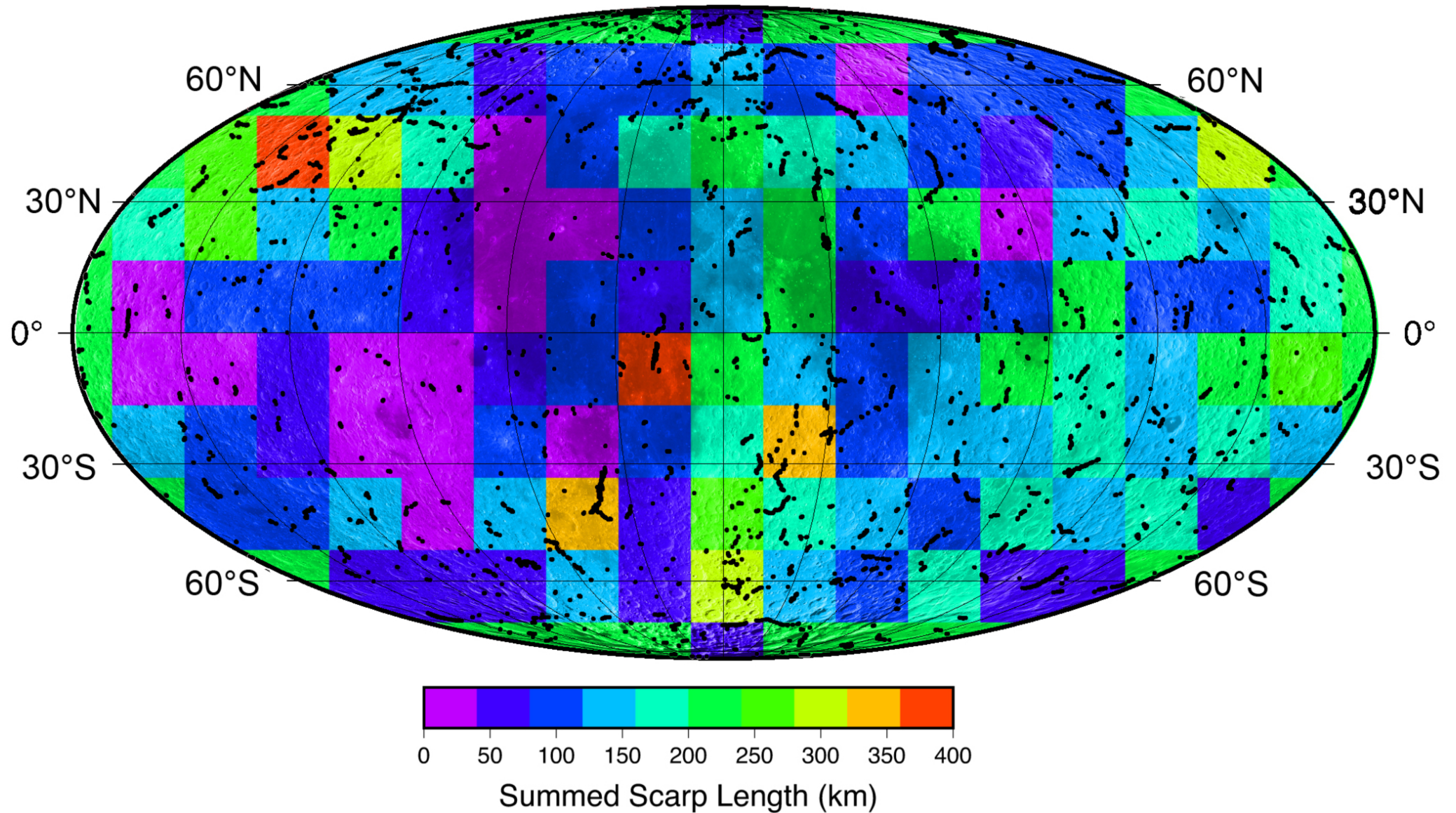
Figure 3. from T. R. Watters et al 2026 Planet. Sci. J. 7 doi:10.3847/PSJ/ae9eae https://dx.doi.org/10.3847/PSJ/ae9eae © 2026. The Author(s). Published by the American Astronomical Society.
