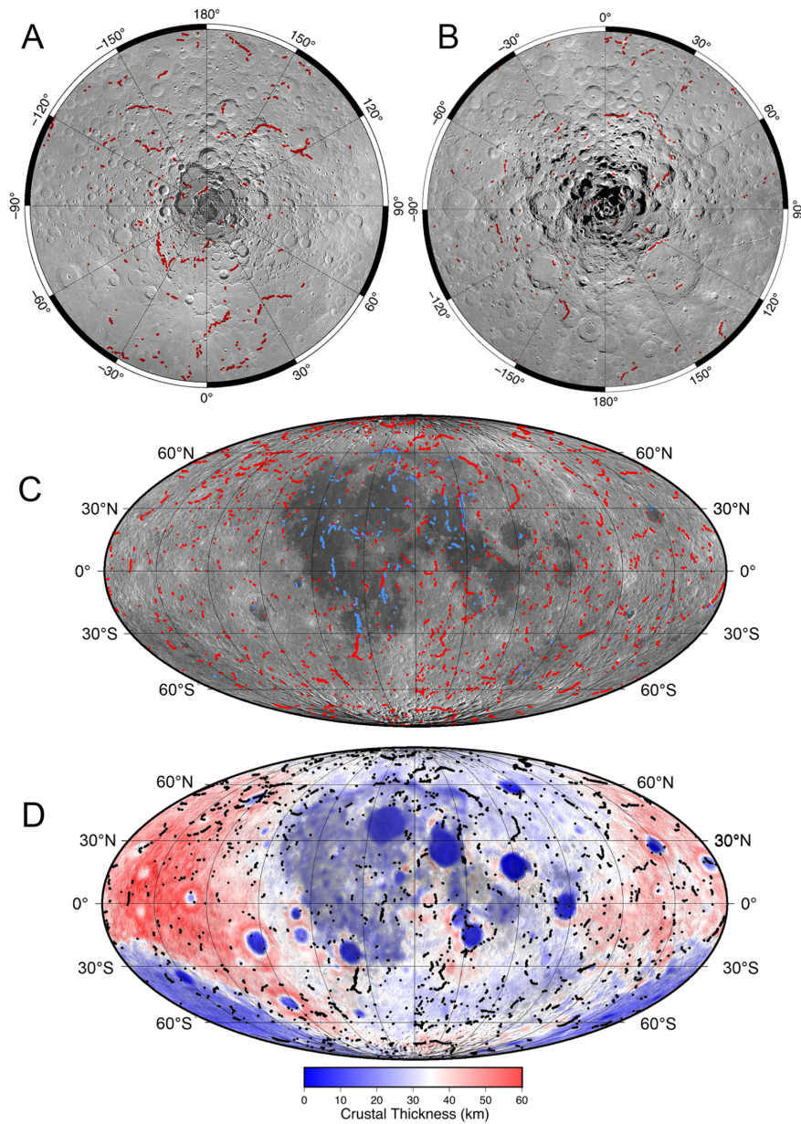
Figure 2. from T. R. Watters et al 2026 Planet. Sci. J. 7 doi:10.3847/PSJ/ae9eae https://dx.doi.org/10.3847/PSJ/ae9eae © 2026. The Author(s). Published by the American Astronomical Society.
