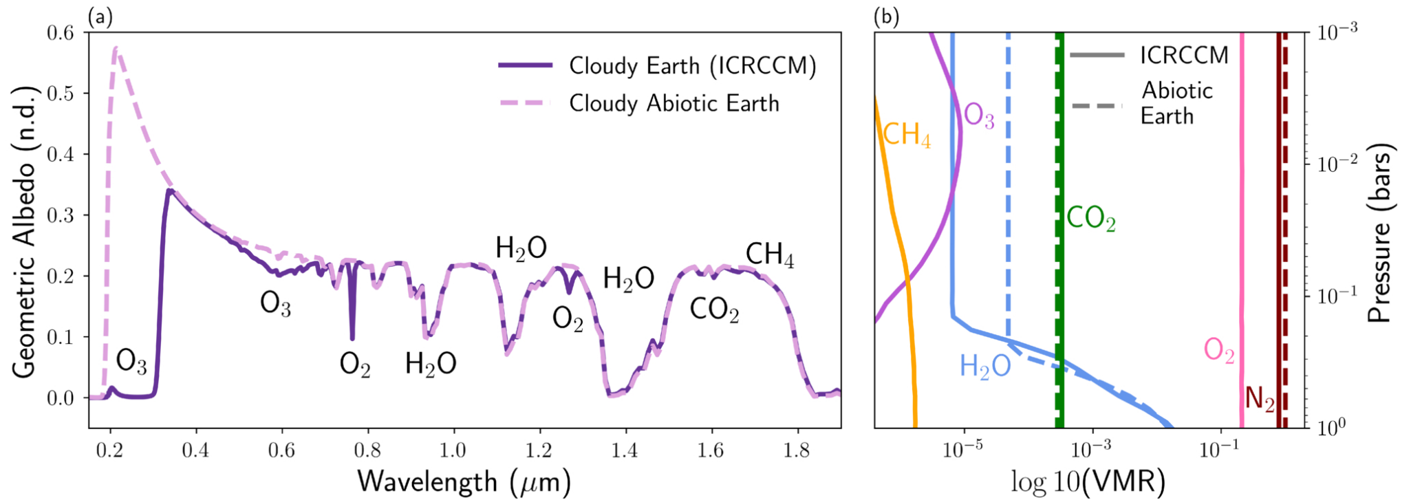
Figure 8. from Samantha Gilbert-Janizek et al 2026 Planet. Sci. J. 7 doi:10.3847/PSJ/ae9d79 https://dx.doi.org/10.3847/PSJ/ae9d79 © 2026. The Author(s). Published by the American Astronomical Society.
