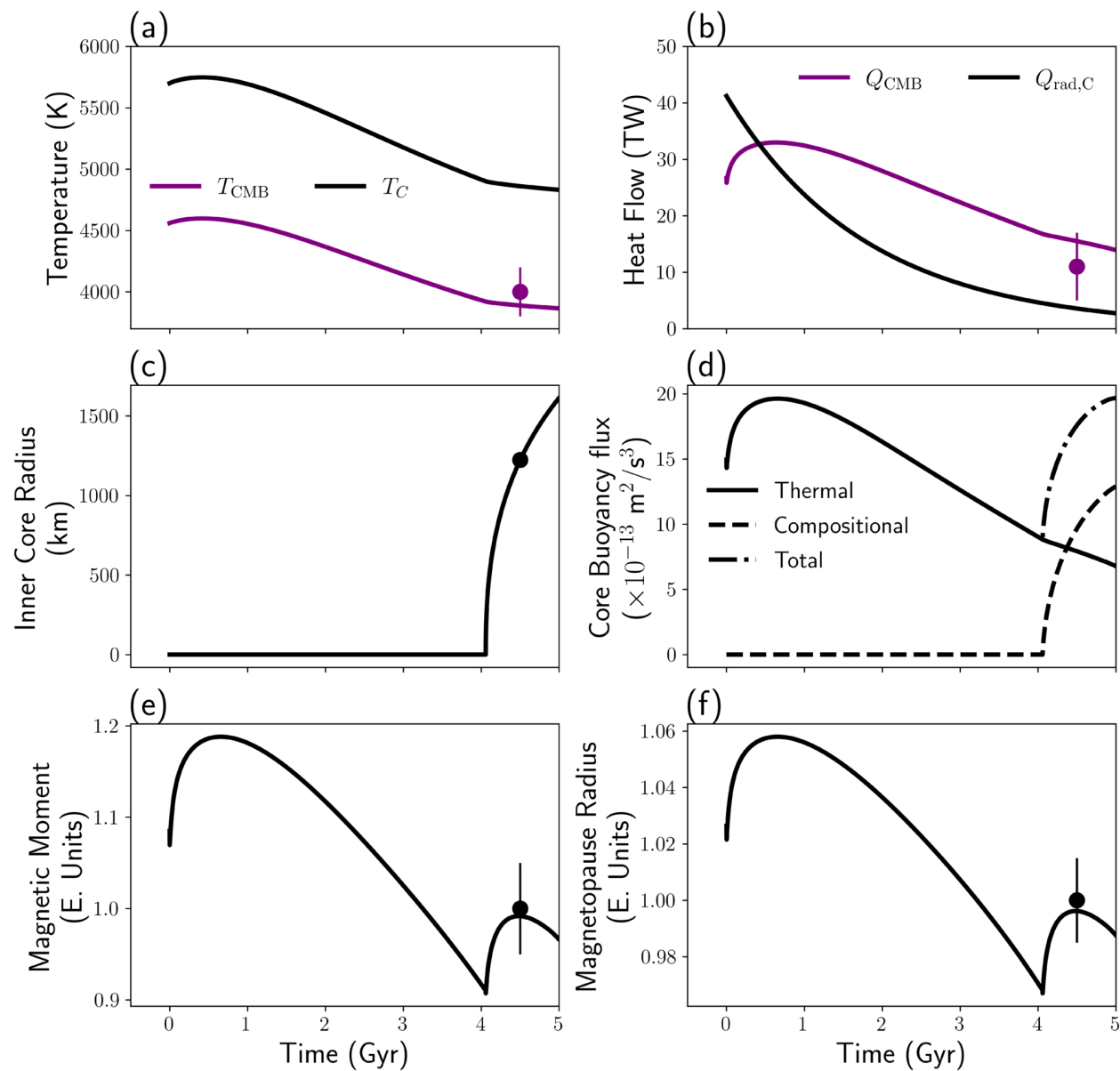
Figure 7. from Samantha Gilbert-Janizek et al 2026 Planet. Sci. J. 7 doi:10.3847/PSJ/ae9d79 https://dx.doi.org/10.3847/PSJ/ae9d79 © 2026. The Author(s). Published by the American Astronomical Society.
