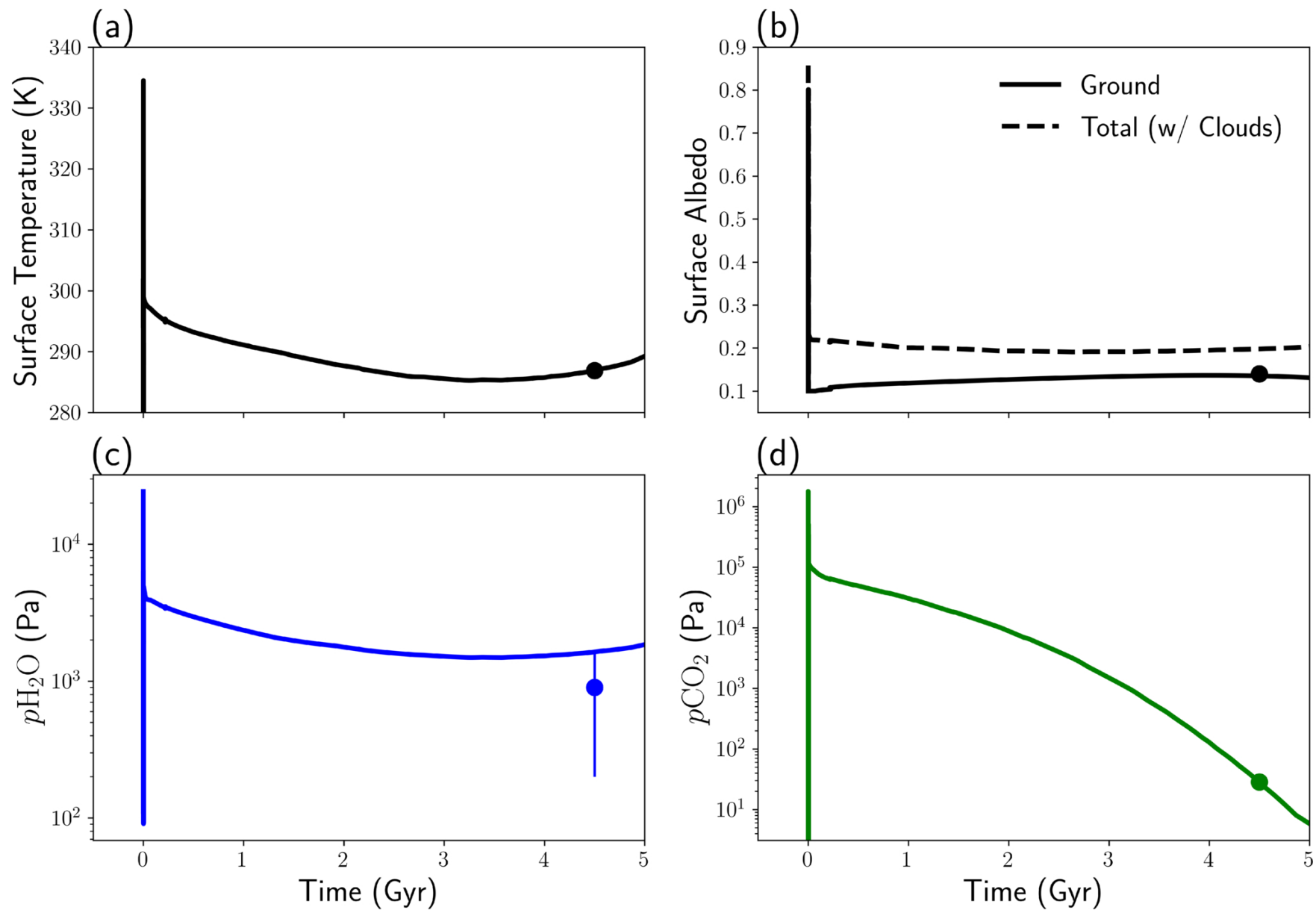
Figure 4. from Samantha Gilbert-Janizek et al 2026 Planet. Sci. J. 7 doi:10.3847/PSJ/ae9d79 https://dx.doi.org/10.3847/PSJ/ae9d79 © 2026. The Author(s). Published by the American Astronomical Society.
