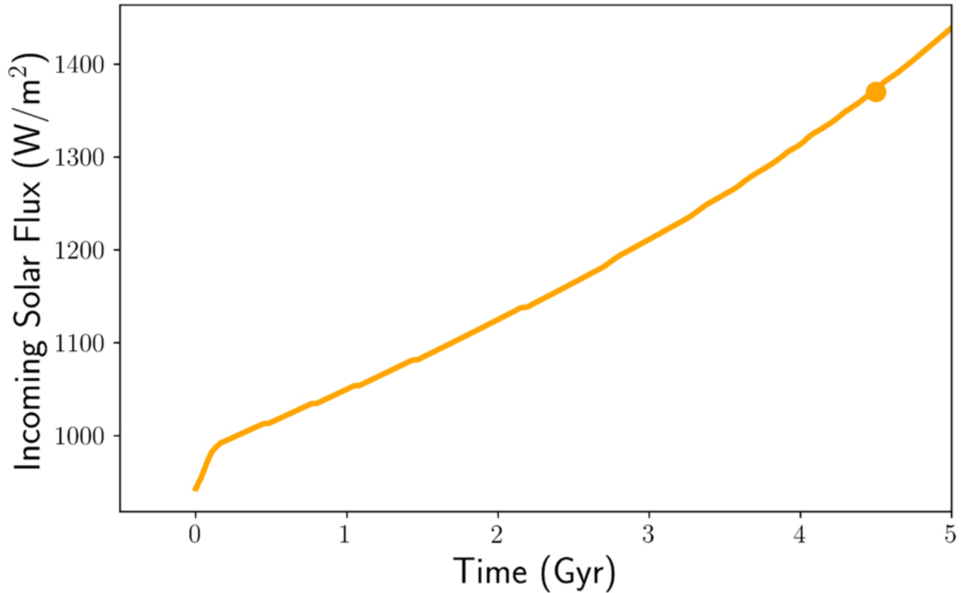
Figure 3. from Samantha Gilbert-Janizek et al 2026 Planet. Sci. J. 7 doi:10.3847/PSJ/ae9d79 https://dx.doi.org/10.3847/PSJ/ae9d79 © 2026. The Author(s). Published by the American Astronomical Society.
