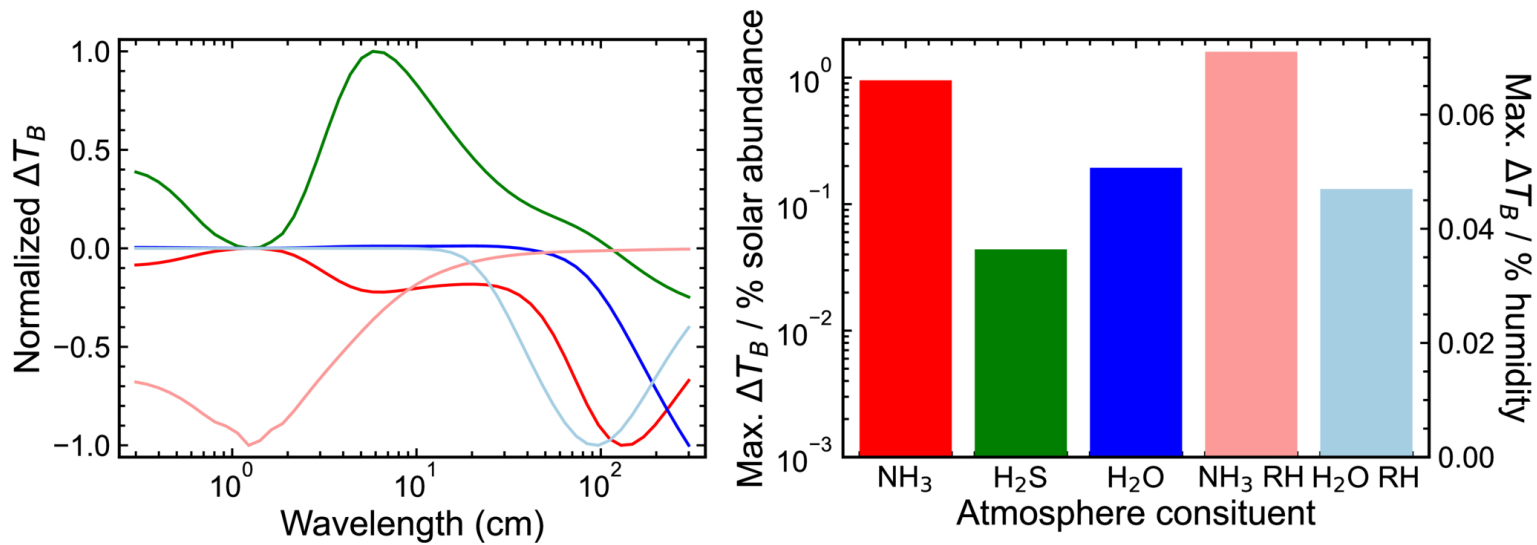
Figure 7. from Alex B. Akins and Mark D. Hofstadter 2026 Planet. Sci. J. 7 doi:10.3847/PSJ/ae9c31 https://dx.doi.org/10.3847/PSJ/ae9c31 © 2026. The Author(s). Published by the American Astronomical Society.
