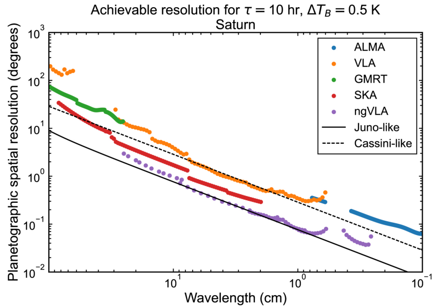
Figure 2. from Alex B. Akins and Mark D. Hofstadter 2026 Planet. Sci. J. 7 doi:10.3847/PSJ/ae9c31 https://dx.doi.org/10.3847/PSJ/ae9c31 © 2026. The Author(s). Published by the American Astronomical Society.
