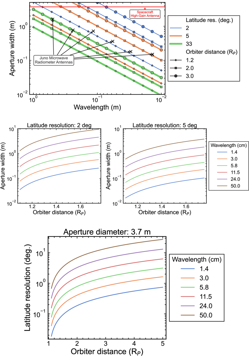
Figure 10. from Alex B. Akins and Mark D. Hofstadter 2026 Planet. Sci. J. 7 doi:10.3847/PSJ/ae9c31 https://dx.doi.org/10.3847/PSJ/ae9c31 © 2026. The Author(s). Published by the American Astronomical Society.
