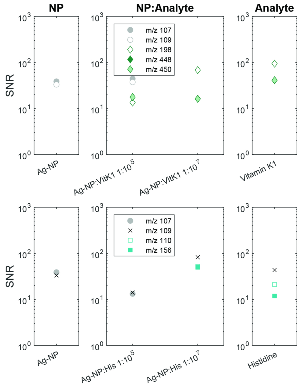
Figure 8. from Nikita J. Boeren et al 2026 Planet. Sci. J. 7 doi:10.3847/PSJ/ae9c2d https://dx.doi.org/10.3847/PSJ/ae9c2d © 2026. The Author(s). Published by the American Astronomical Society.
