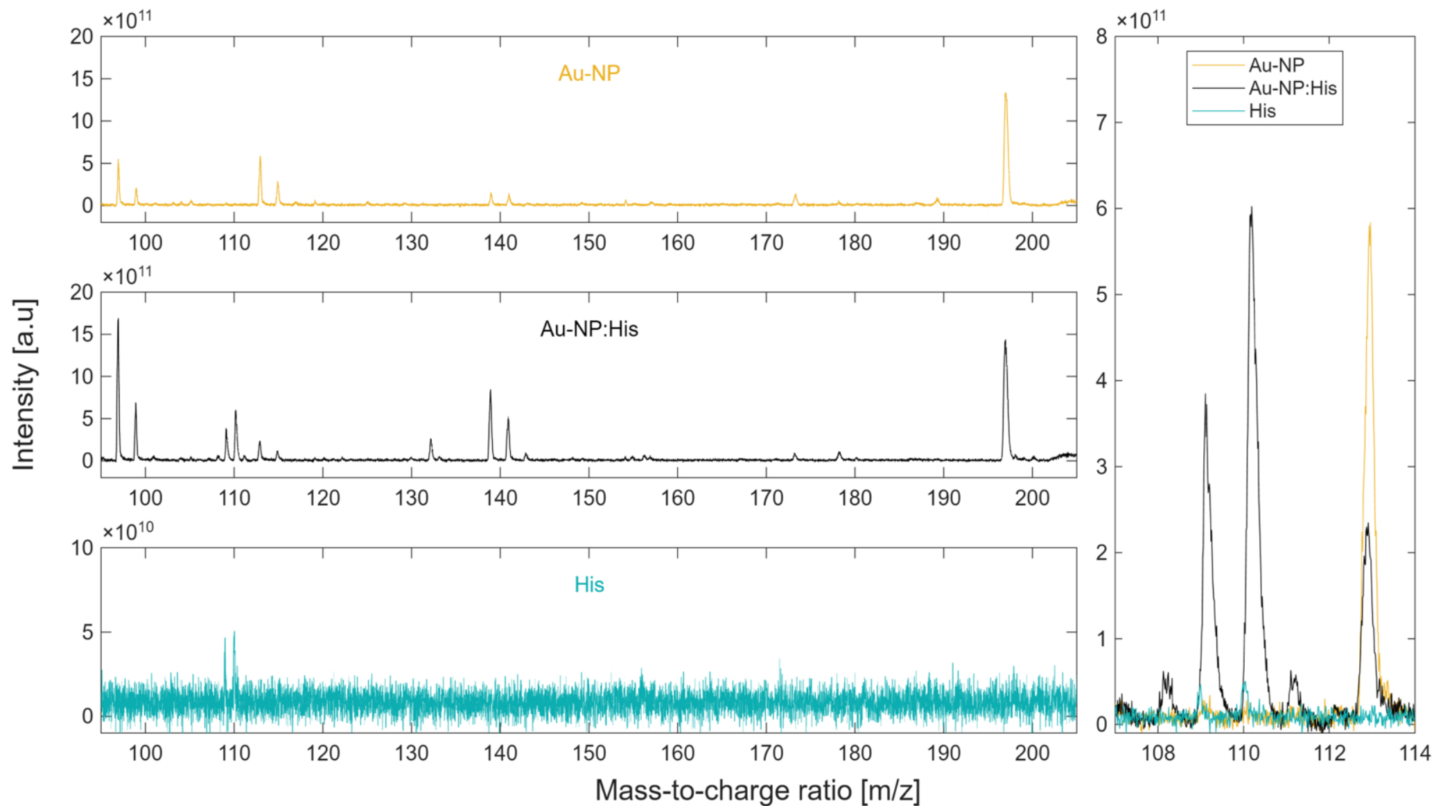
Figure 3. from Nikita J. Boeren et al 2026 Planet. Sci. J. 7 doi:10.3847/PSJ/ae9c2d https://dx.doi.org/10.3847/PSJ/ae9c2d © 2026. The Author(s). Published by the American Astronomical Society.
