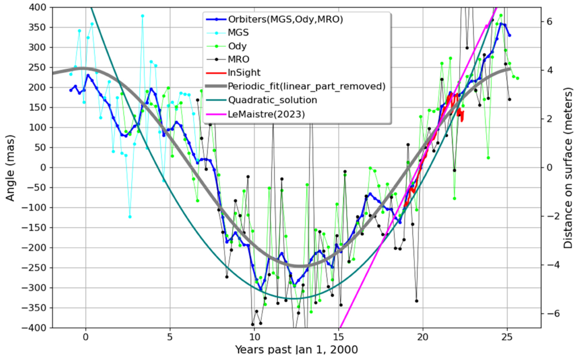
Figure 7. from Alex. S. Konopliv et al 2026 Planet. Sci. J. 7 doi:10.3847/PSJ/ae9ba7 https://dx.doi.org/10.3847/PSJ/ae9ba7 © 2026. The Author(s). Published by the American Astronomical Society.
