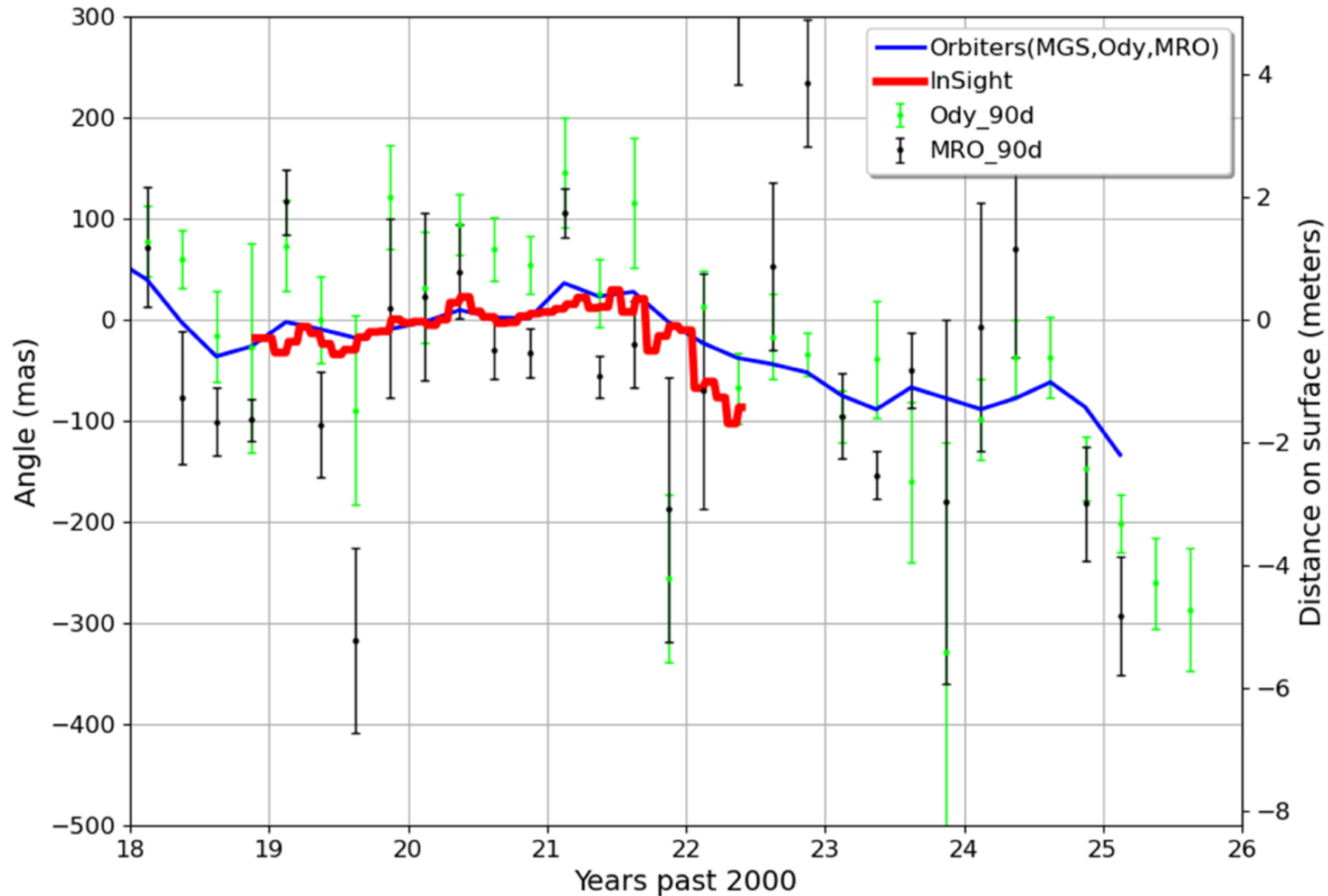
Figure 6. from Alex. S. Konopliv et al 2026 Planet. Sci. J. 7 doi:10.3847/PSJ/ae9ba7 https://dx.doi.org/10.3847/PSJ/ae9ba7 © 2026. The Author(s). Published by the American Astronomical Society.
