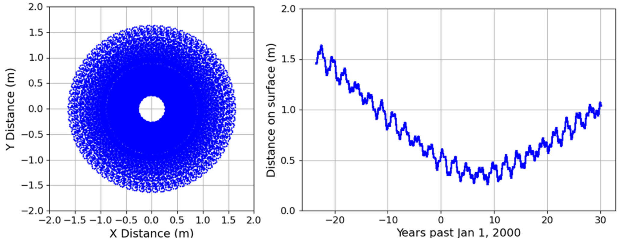
Figure 3. from Alex. S. Konopliv et al 2026 Planet. Sci. J. 7 doi:10.3847/PSJ/ae9ba7 https://dx.doi.org/10.3847/PSJ/ae9ba7 © 2026. The Author(s). Published by the American Astronomical Society.
