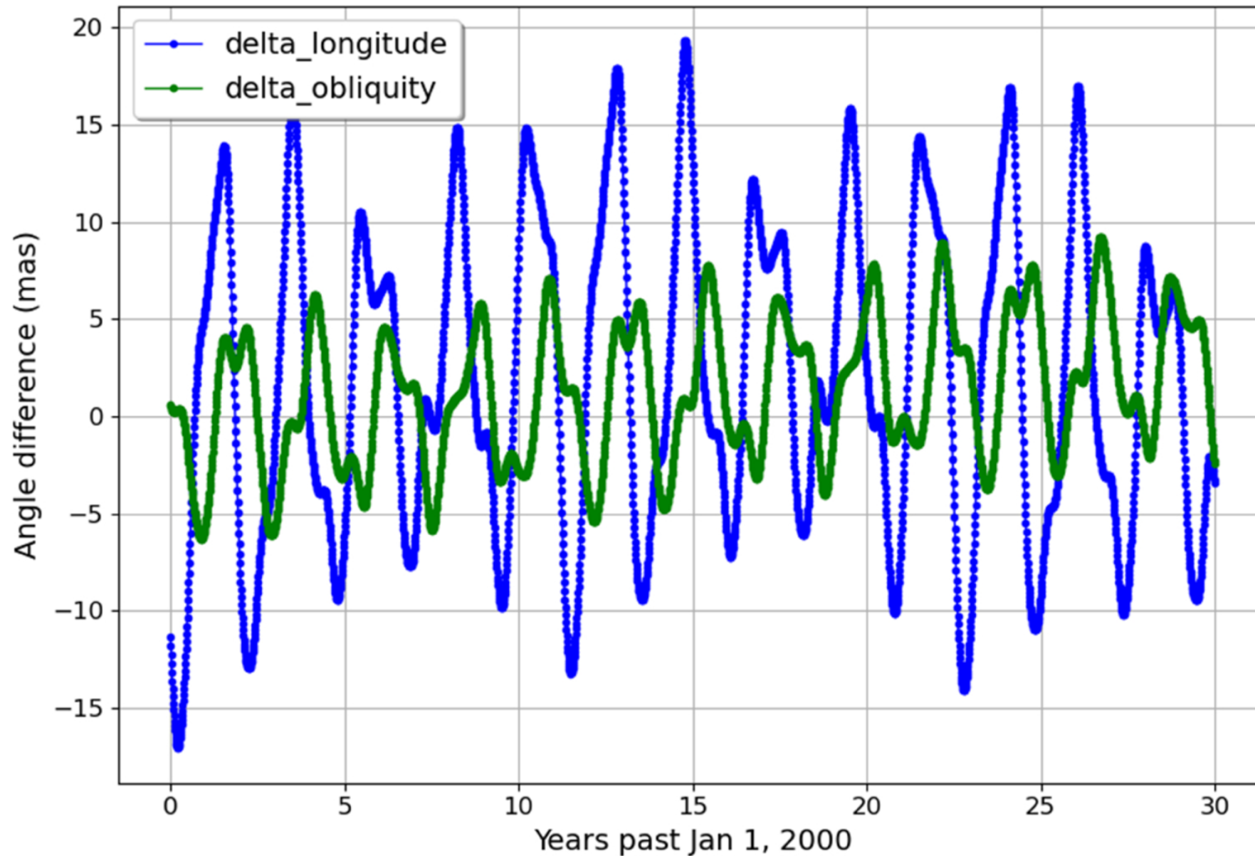
Figure 2. from Alex. S. Konopliv et al 2026 Planet. Sci. J. 7 doi:10.3847/PSJ/ae9ba7 https://dx.doi.org/10.3847/PSJ/ae9ba7 © 2026. The Author(s). Published by the American Astronomical Society.
