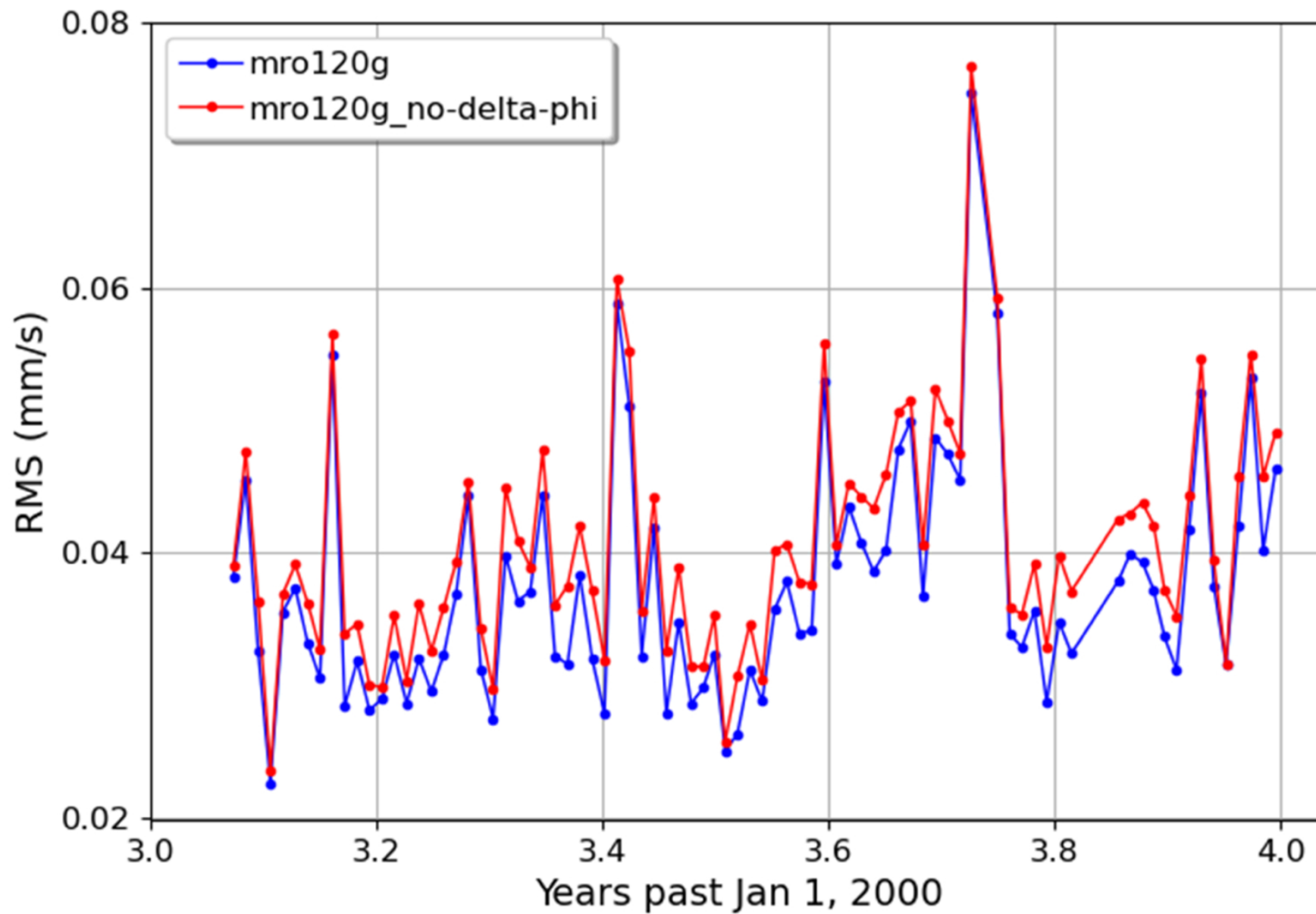
Figure A3. from Alex. S. Konopliv et al 2026 Planet. Sci. J. 7 doi:10.3847/PSJ/ae9ba7 https://dx.doi.org/10.3847/PSJ/ae9ba7 © 2026. The Author(s). Published by the American Astronomical Society.
