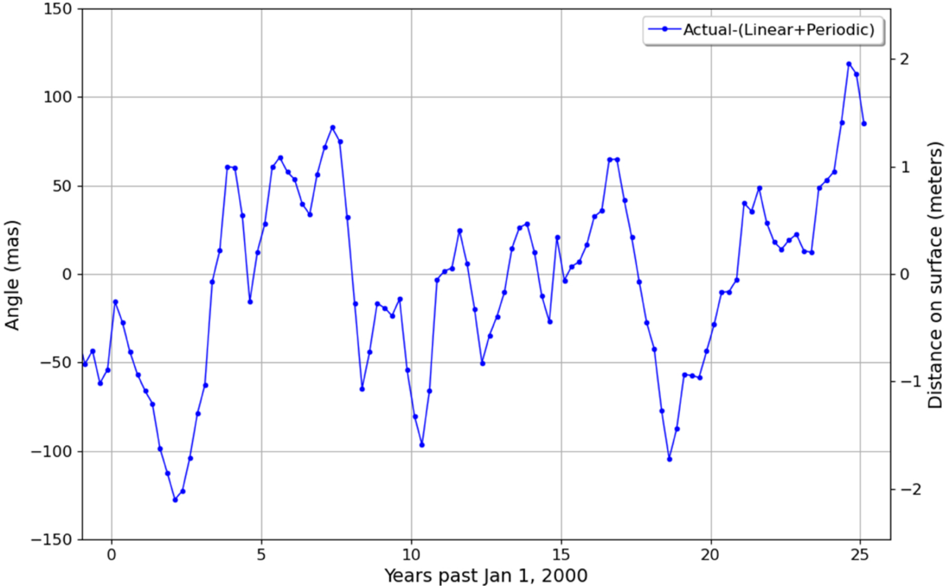
Figure A2. from Alex. S. Konopliv et al 2026 Planet. Sci. J. 7 doi:10.3847/PSJ/ae9ba7 https://dx.doi.org/10.3847/PSJ/ae9ba7 © 2026. The Author(s). Published by the American Astronomical Society.
