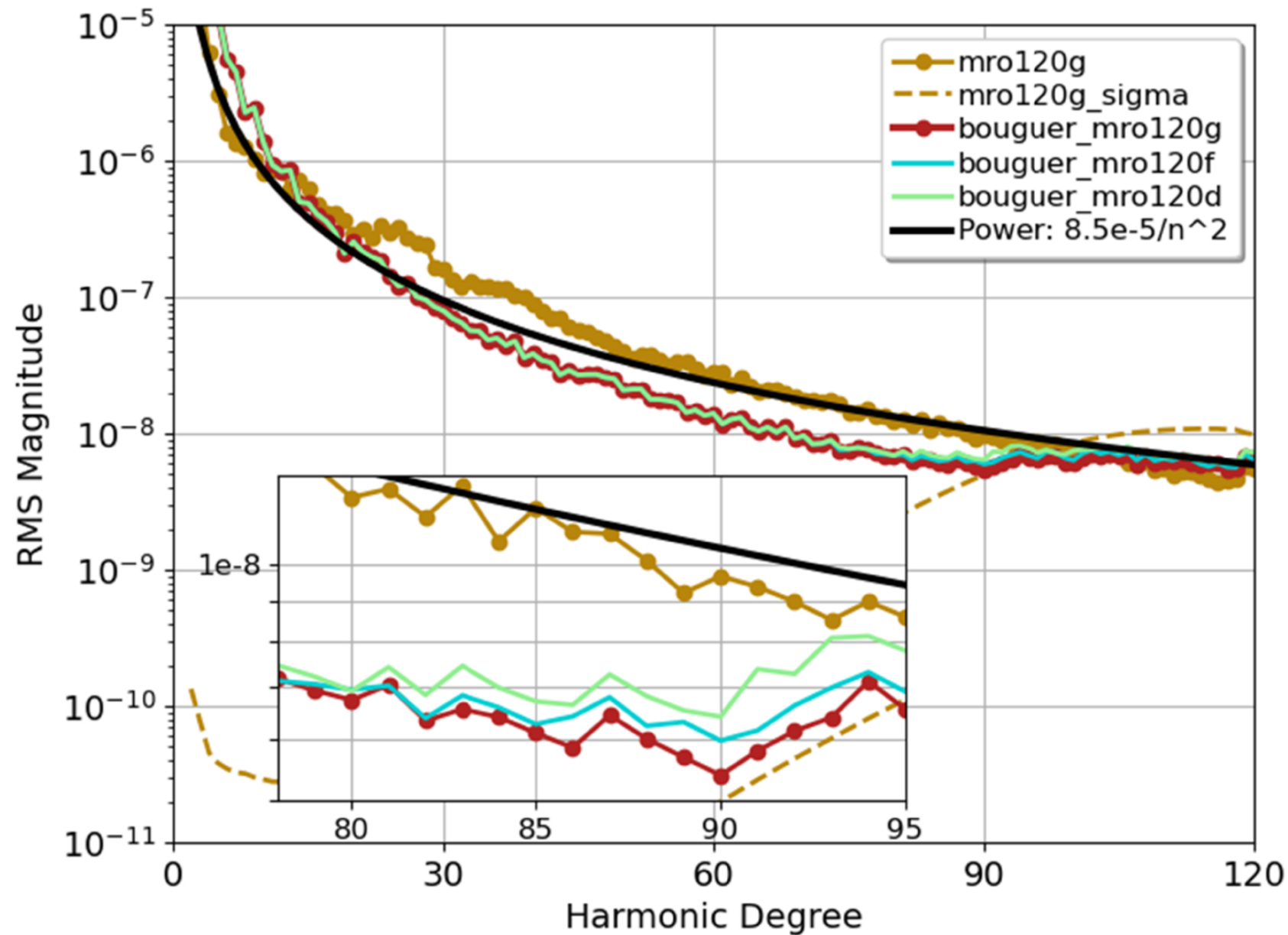
Figure 10. from Alex. S. Konopliv et al 2026 Planet. Sci. J. 7 doi:10.3847/PSJ/ae9ba7 https://dx.doi.org/10.3847/PSJ/ae9ba7 © 2026. The Author(s). Published by the American Astronomical Society.
