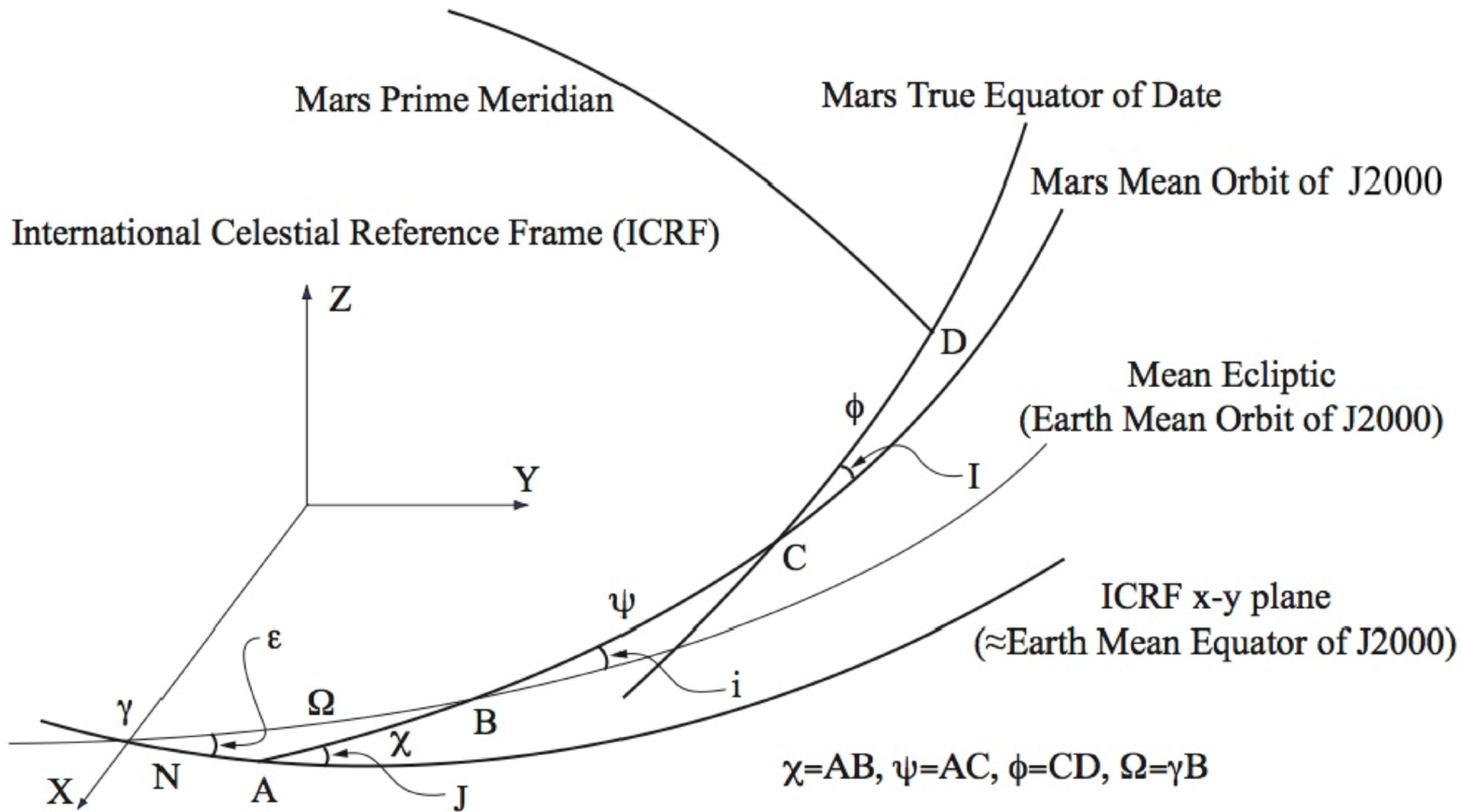
Figure 1. from Alex. S. Konopliv et al 2026 Planet. Sci. J. 7 doi:10.3847/PSJ/ae9ba7 https://dx.doi.org/10.3847/PSJ/ae9ba7 © 2026. The Author(s). Published by the American Astronomical Society.
