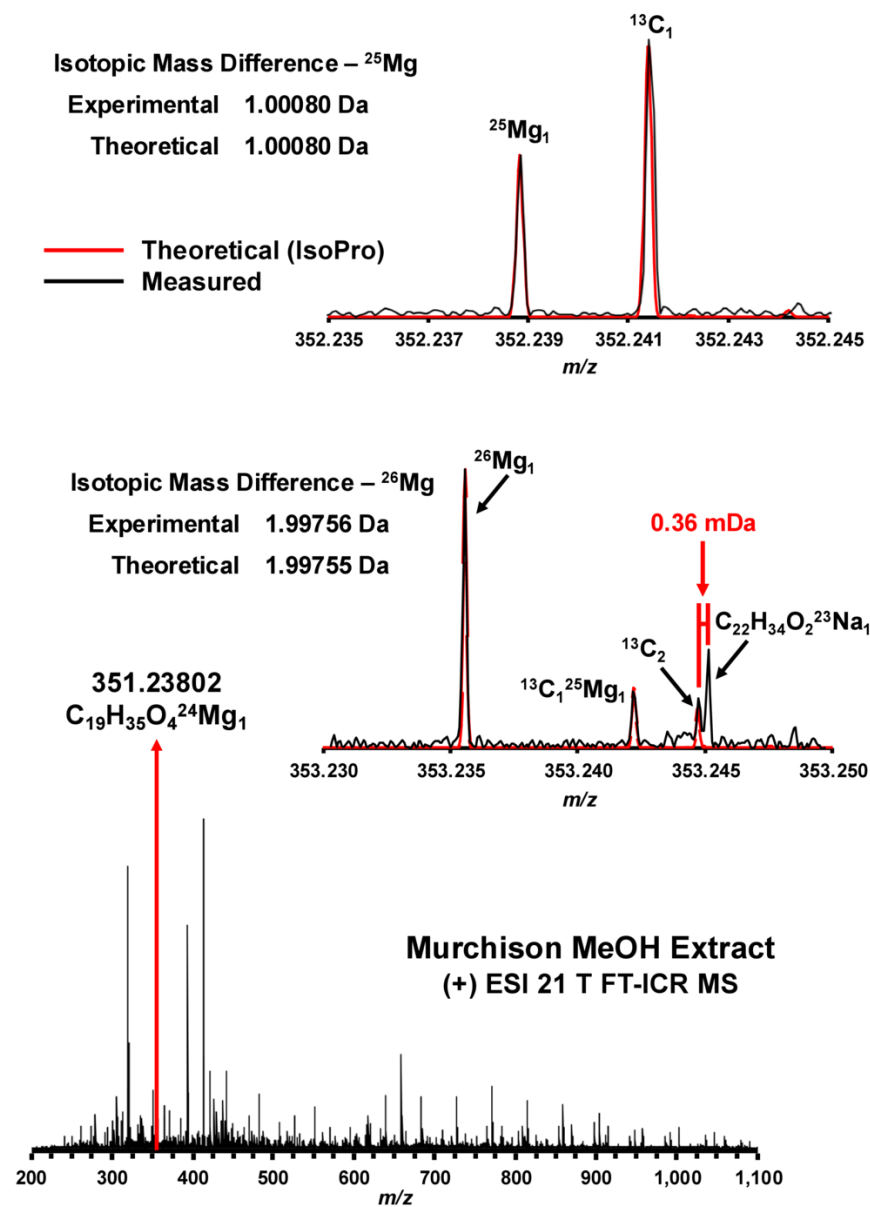
Figure 7. from Joseph W. Frye-Jones et al 2026 Planet. Sci. J. 7 doi:10.3847/PSJ/ae9a8d https://dx.doi.org/10.3847/PSJ/ae9a8d © 2026. The Author(s). Published by the American Astronomical Society.
