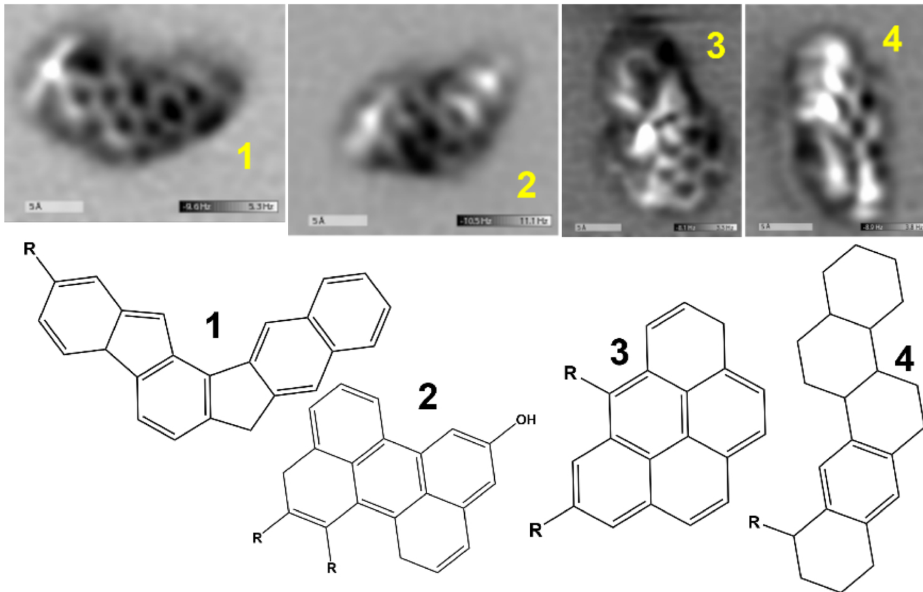
Figure C2. from Joseph W. Frye-Jones et al 2026 Planet. Sci. J. 7 doi:10.3847/PSJ/ae9a8d https://dx.doi.org/10.3847/PSJ/ae9a8d © 2026. The Author(s). Published by the American Astronomical Society.
