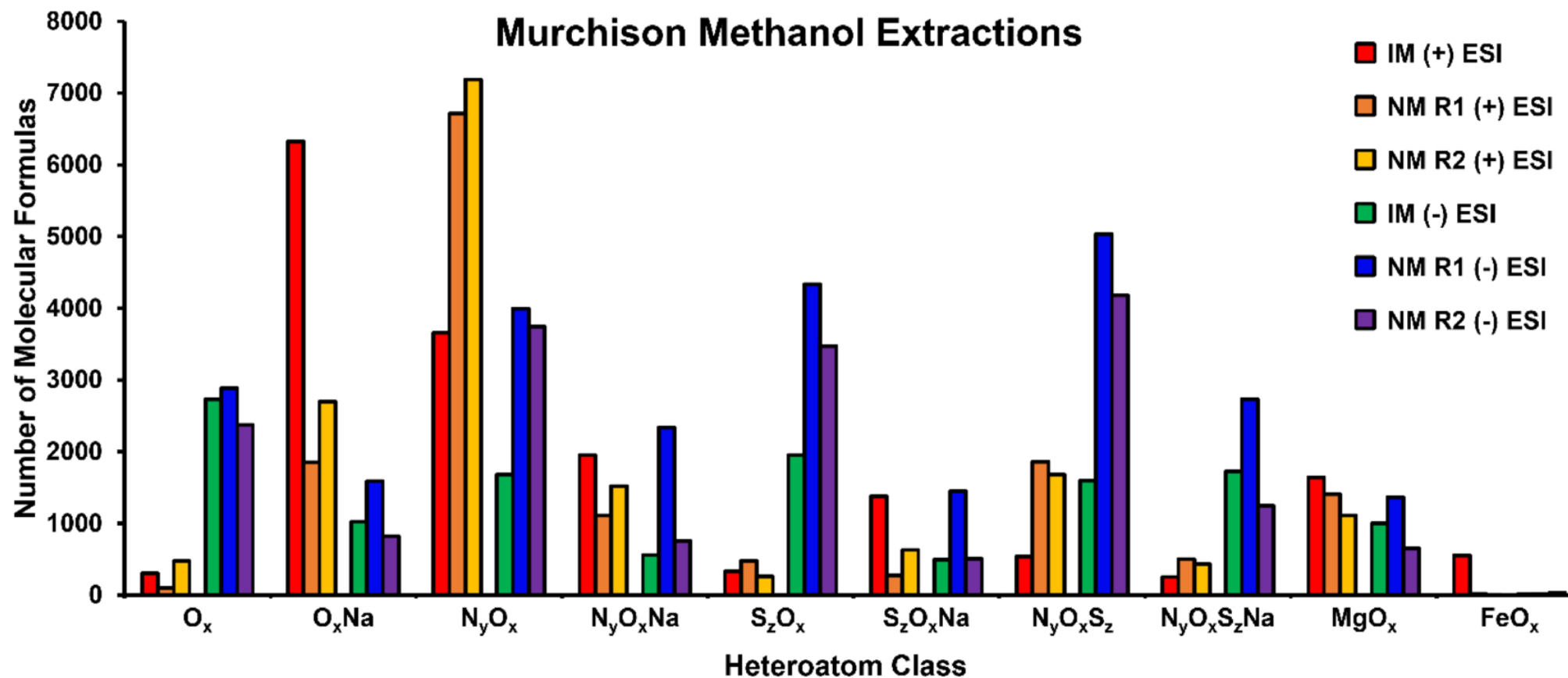
Figure A3. from Joseph W. Frye-Jones et al 2026 Planet. Sci. J. 7 doi:10.3847/PSJ/ae9a8d https://dx.doi.org/10.3847/PSJ/ae9a8d © 2026. The Author(s). Published by the American Astronomical Society.
