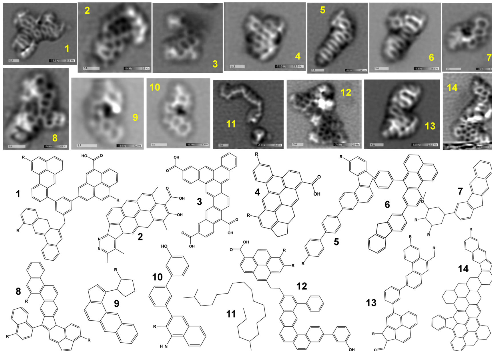
Figure 10. from Joseph W. Frye-Jones et al 2026 Planet. Sci. J. 7 doi:10.3847/PSJ/ae9a8d https://dx.doi.org/10.3847/PSJ/ae9a8d © 2026. The Author(s). Published by the American Astronomical Society.
