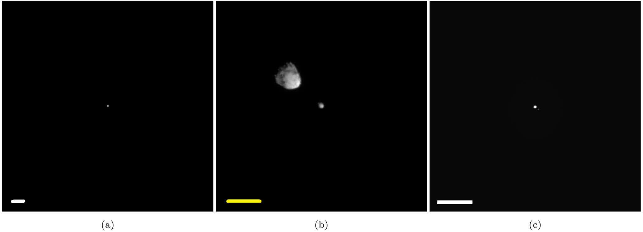
Figure 1. from Ivano Bertini et al 2026 Planet. Sci. J. 7 doi:10.3847/PSJ/ae99e5 https://dx.doi.org/10.3847/PSJ/ae99e5 © 2026. The Author(s). Published by the American Astronomical Society.
