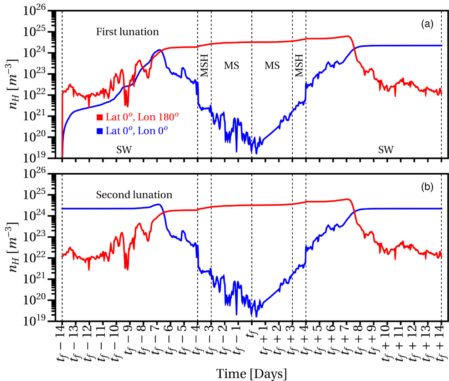
Figure 9. from Trinesh Sana and S. K. Mishra 2026 Planet. Sci. J. 7 doi:10.3847/PSJ/ae9951 https://dx.doi.org/10.3847/PSJ/ae9951 © 2026. The Author(s). Published by the American Astronomical Society.
