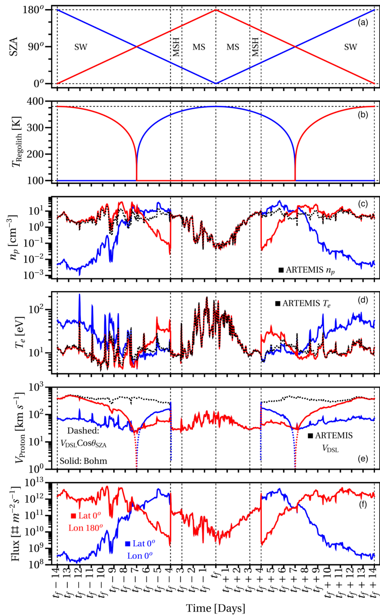
Figure 8. from Trinesh Sana and S. K. Mishra 2026 Planet. Sci. J. 7 doi:10.3847/PSJ/ae9951 https://dx.doi.org/10.3847/PSJ/ae9951 © 2026. The Author(s). Published by the American Astronomical Society.
