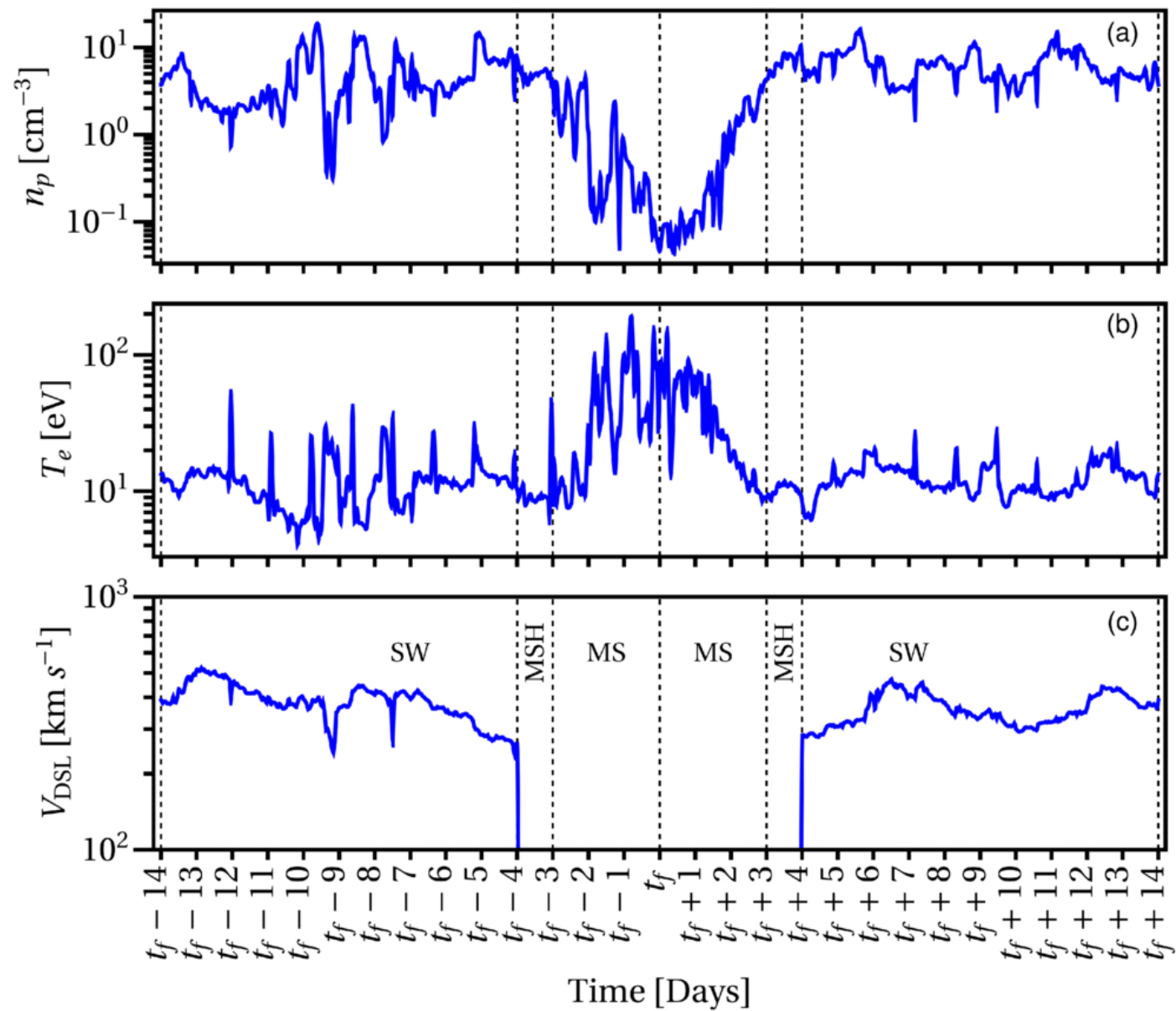
Figure 7. from Trinesh Sana and S. K. Mishra 2026 Planet. Sci. J. 7 doi:10.3847/PSJ/ae9951 https://dx.doi.org/10.3847/PSJ/ae9951 © 2026. The Author(s). Published by the American Astronomical Society.
