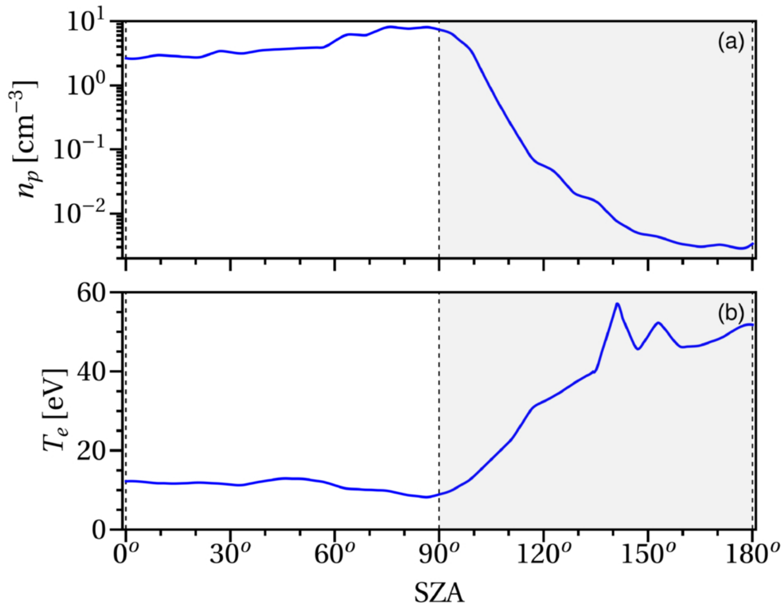
Figure 6. from Trinesh Sana and S. K. Mishra 2026 Planet. Sci. J. 7 doi:10.3847/PSJ/ae9951 https://dx.doi.org/10.3847/PSJ/ae9951 © 2026. The Author(s). Published by the American Astronomical Society.
