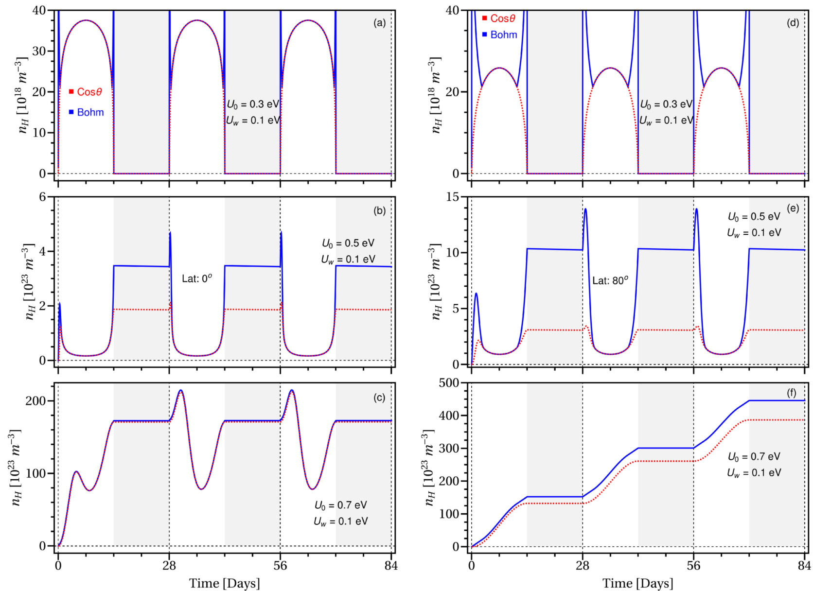
Figure 5. from Trinesh Sana and S. K. Mishra 2026 Planet. Sci. J. 7 doi:10.3847/PSJ/ae9951 https://dx.doi.org/10.3847/PSJ/ae9951 © 2026. The Author(s). Published by the American Astronomical Society.
