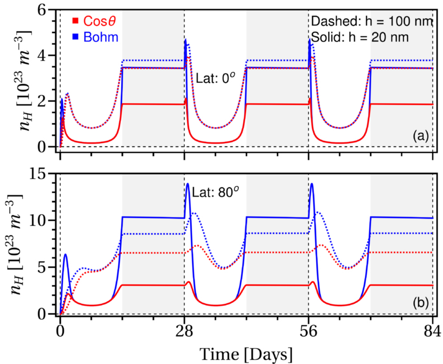
Figure 4. from Trinesh Sana and S. K. Mishra 2026 Planet. Sci. J. 7 doi:10.3847/PSJ/ae9951 https://dx.doi.org/10.3847/PSJ/ae9951 © 2026. The Author(s). Published by the American Astronomical Society.
