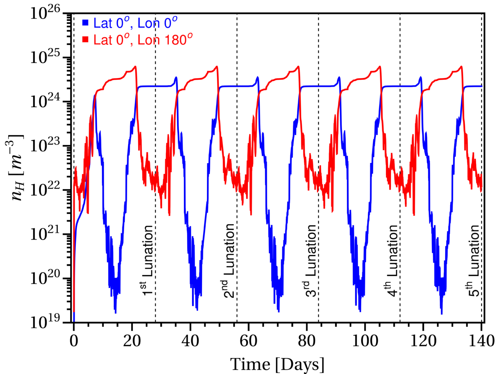
Figure C3. from Trinesh Sana and S. K. Mishra 2026 Planet. Sci. J. 7 doi:10.3847/PSJ/ae9951 https://dx.doi.org/10.3847/PSJ/ae9951 © 2026. The Author(s). Published by the American Astronomical Society.
