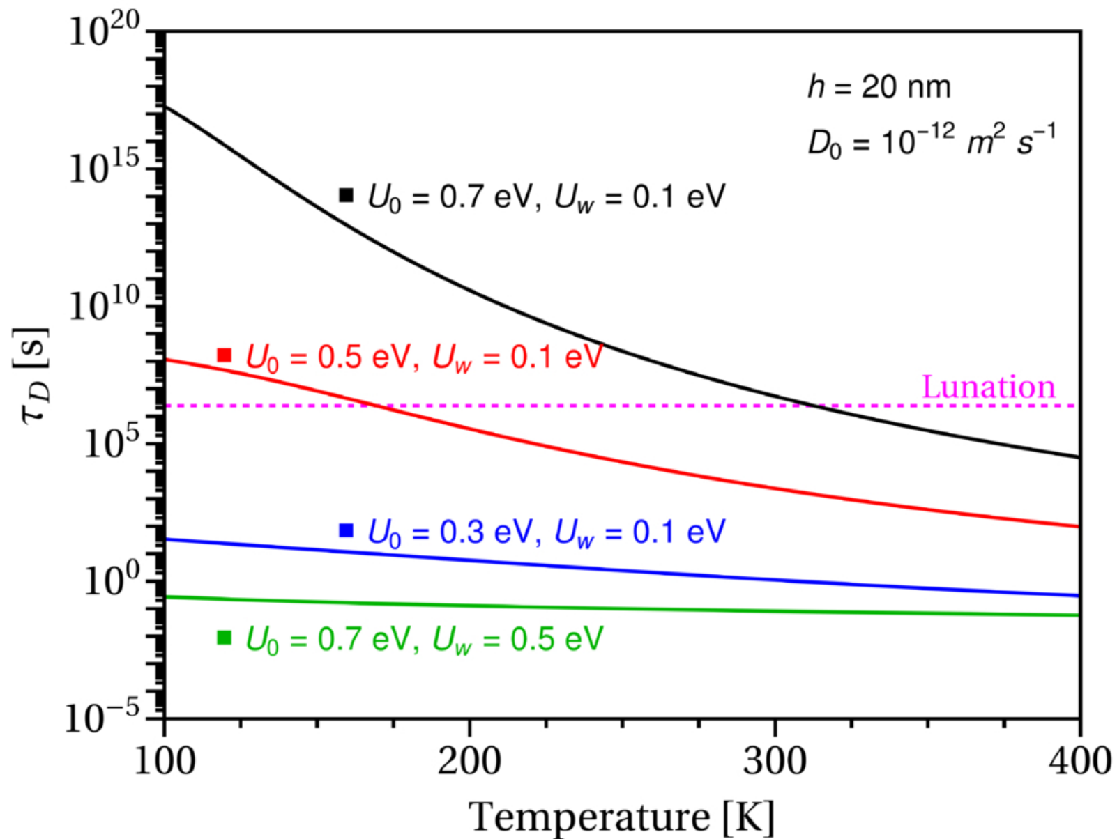
Figure C2. from Trinesh Sana and S. K. Mishra 2026 Planet. Sci. J. 7 doi:10.3847/PSJ/ae9951 https://dx.doi.org/10.3847/PSJ/ae9951 © 2026. The Author(s). Published by the American Astronomical Society.
