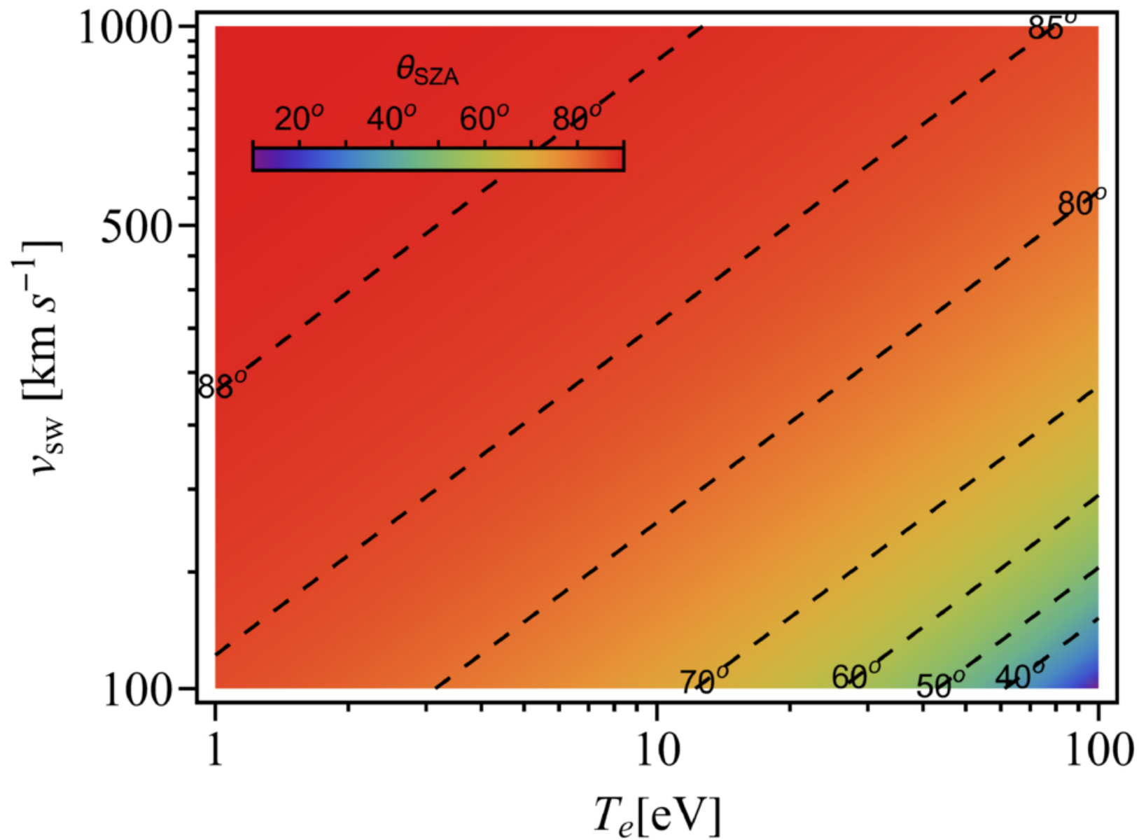
Figure C1. from Trinesh Sana and S. K. Mishra 2026 Planet. Sci. J. 7 doi:10.3847/PSJ/ae9951 https://dx.doi.org/10.3847/PSJ/ae9951 © 2026. The Author(s). Published by the American Astronomical Society.
