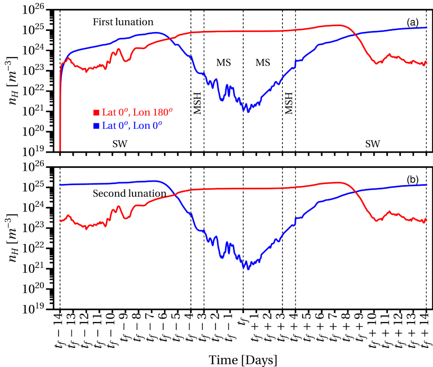
Figure 10. from Trinesh Sana and S. K. Mishra 2026 Planet. Sci. J. 7 doi:10.3847/PSJ/ae9951 https://dx.doi.org/10.3847/PSJ/ae9951 © 2026. The Author(s). Published by the American Astronomical Society.
