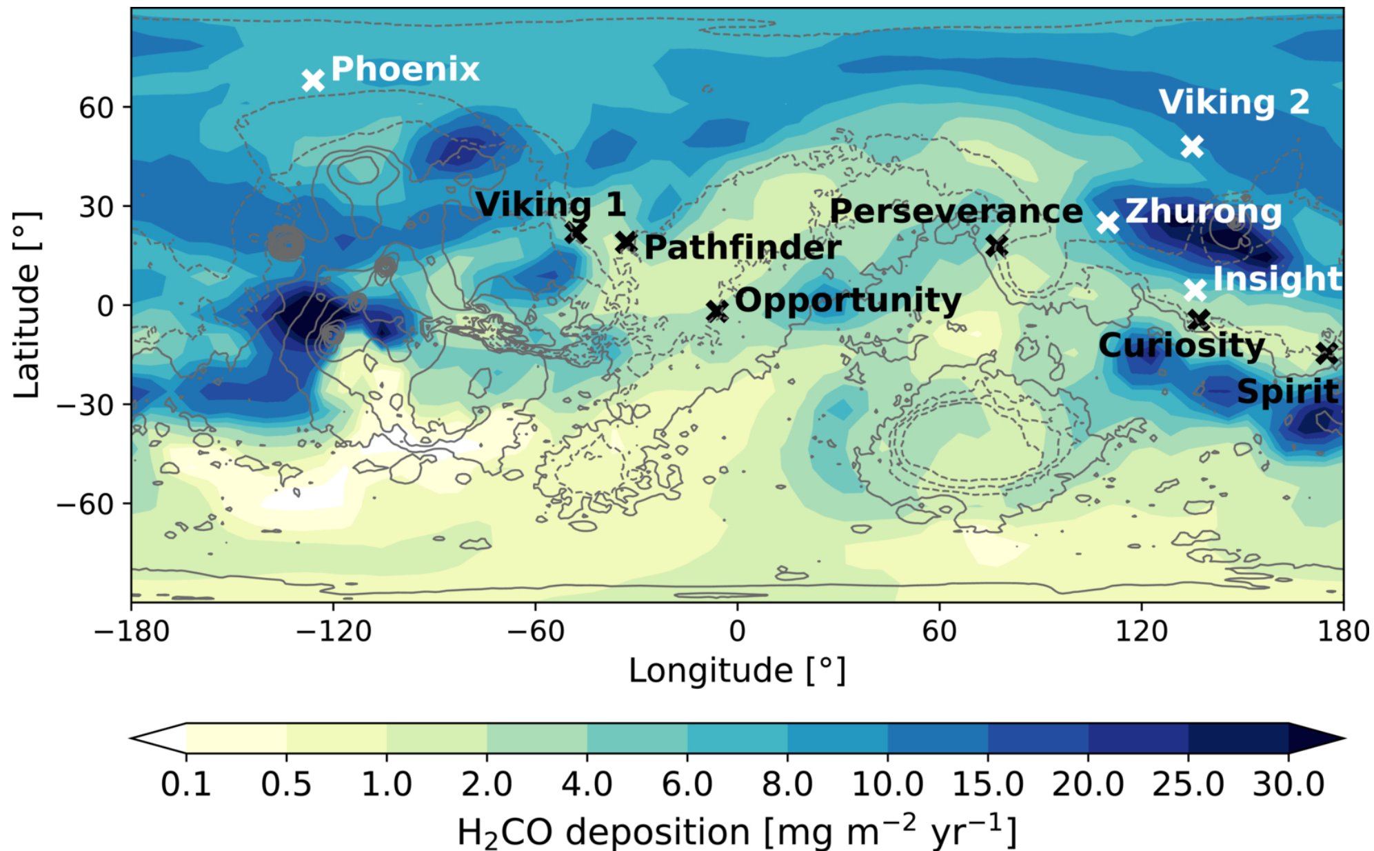
Figure 6. from Shungo Koyama et al 2026 Planet. Sci. J. 7 doi:10.3847/PSJ/ae9942 https://dx.doi.org/10.3847/PSJ/ae9942 © 2026. The Author(s). Published by the American Astronomical Society.
