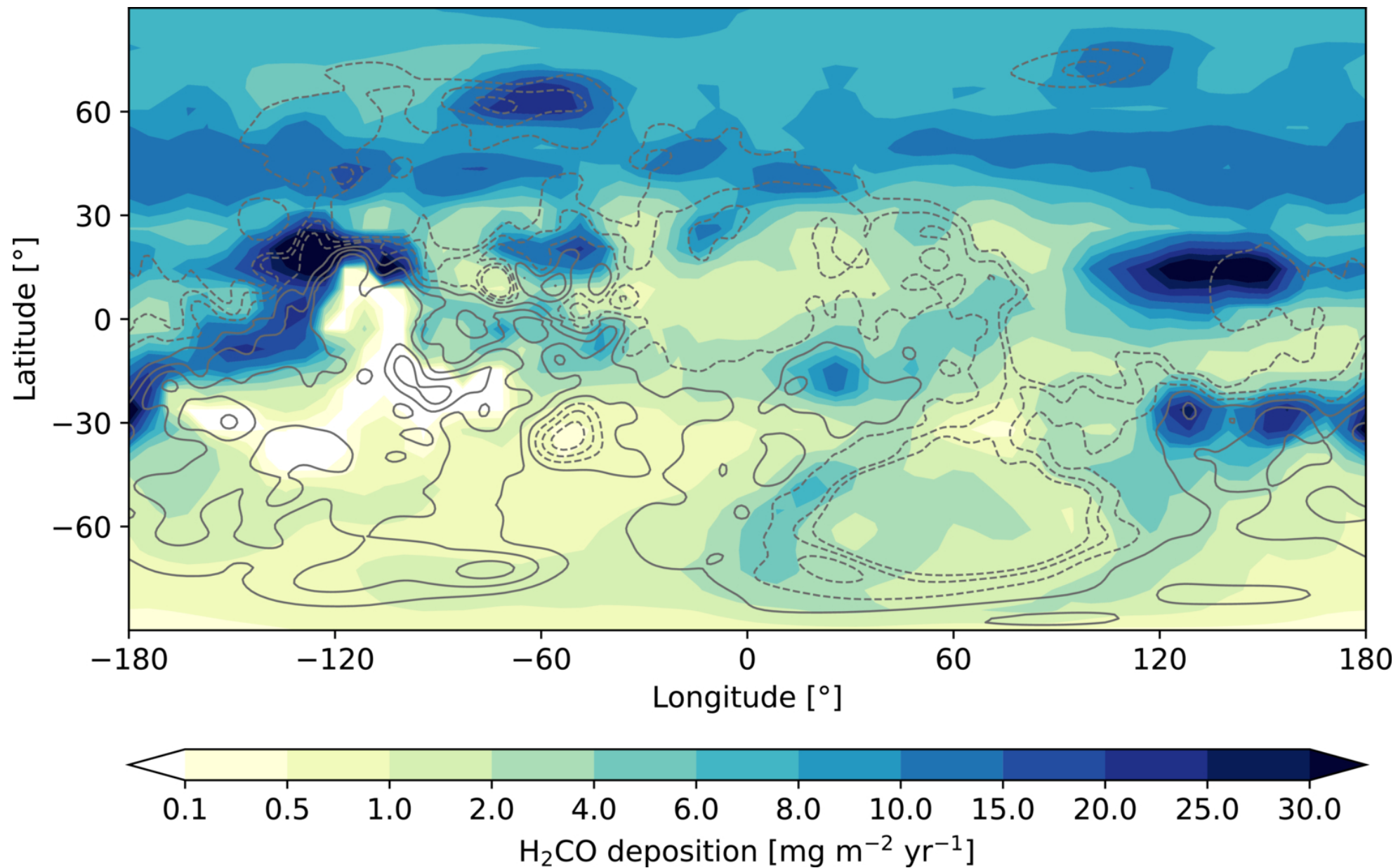
Figure 5. from Shungo Koyama et al 2026 Planet. Sci. J. 7 doi:10.3847/PSJ/ae9942 https://dx.doi.org/10.3847/PSJ/ae9942 © 2026. The Author(s). Published by the American Astronomical Society.
