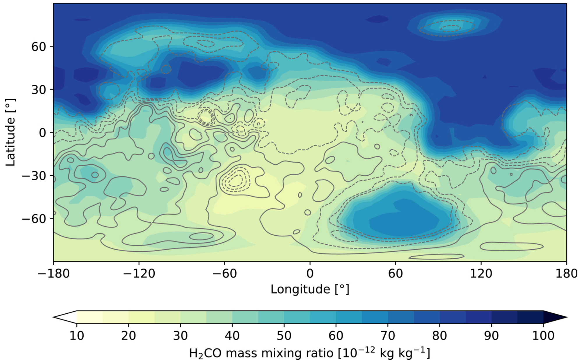
Figure 4. from Shungo Koyama et al 2026 Planet. Sci. J. 7 doi:10.3847/PSJ/ae9942 https://dx.doi.org/10.3847/PSJ/ae9942 © 2026. The Author(s). Published by the American Astronomical Society.
