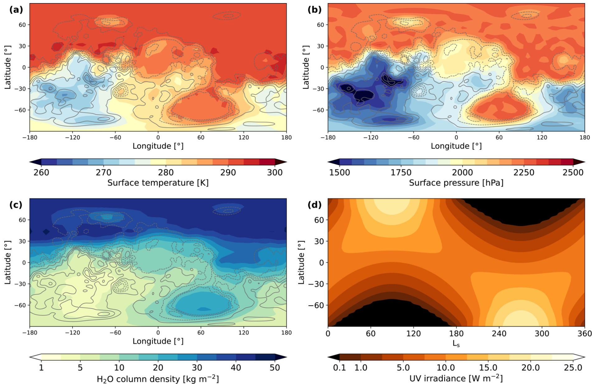
Figure 2. from Shungo Koyama et al 2026 Planet. Sci. J. 7 doi:10.3847/PSJ/ae9942 https://dx.doi.org/10.3847/PSJ/ae9942 © 2026. The Author(s). Published by the American Astronomical Society.
