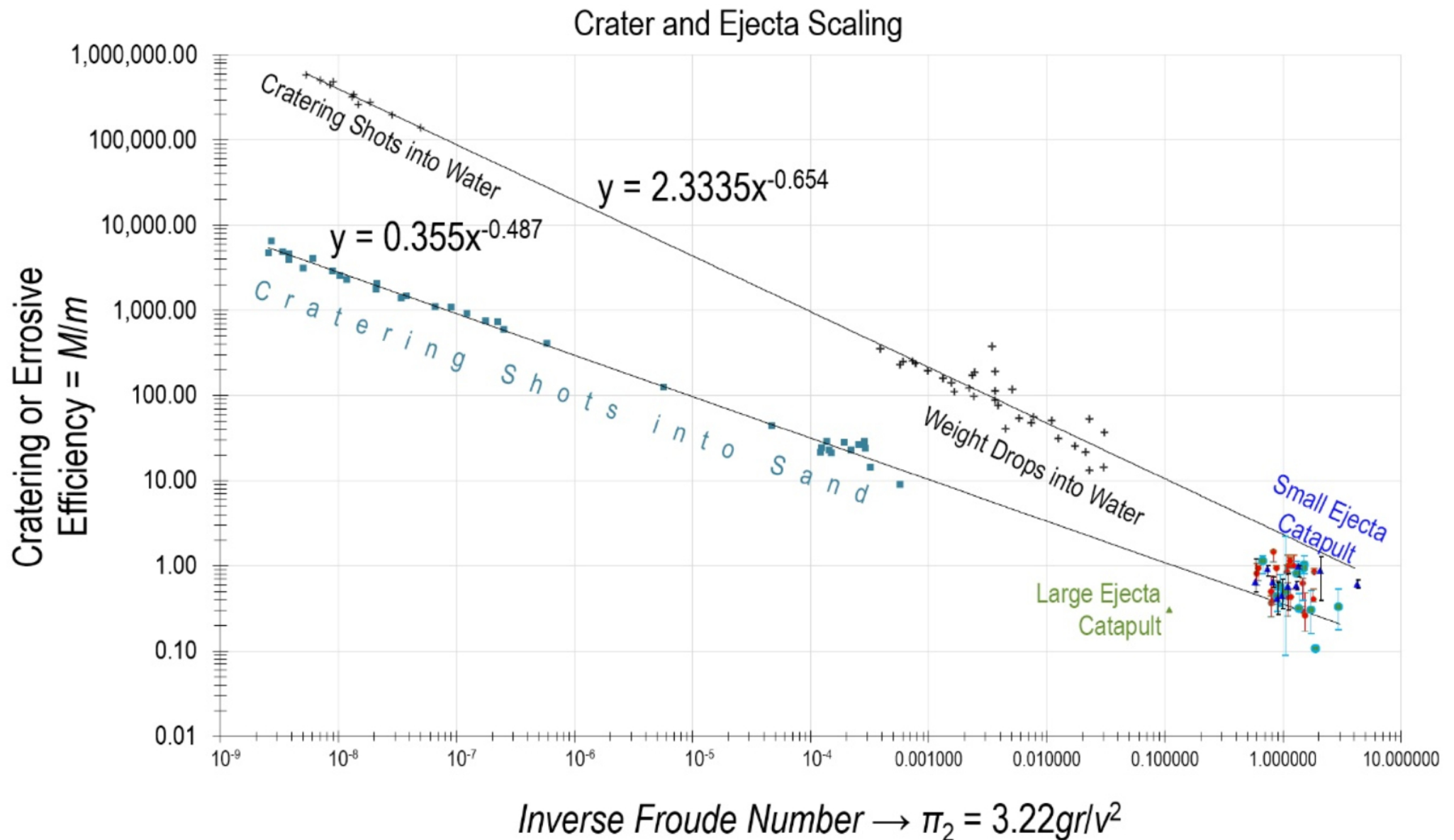
Figure 9. from Kirby D. Runyon et al 2026 Planet. Sci. J. 7 doi:10.3847/PSJ/ae9875 https://dx.doi.org/10.3847/PSJ/ae9875 © 2026. The Author(s). Published by the American Astronomical Society.
